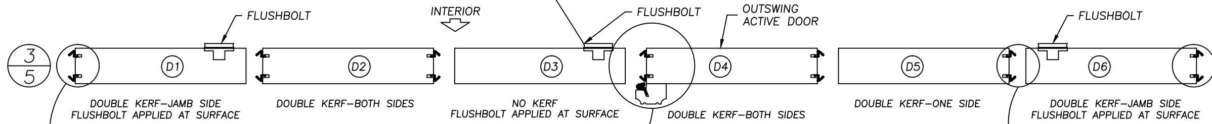
② HORIZONTAL CROSS SECTION ⑤ MIDDLE OF DOOR. VIEWED FROM TOP RAIL HALF OFFSET WITH HANDLE TO PULL INTERIOR SIDE
