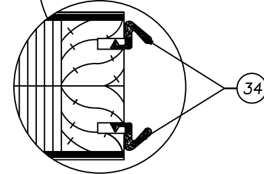
WEATHERSTRIP DETAIL DOORS D1,D3,D4,D5,D6 HAVE (1) EDGES EACH KERFED FOR WEATHERSTRIP (2) PLACES
