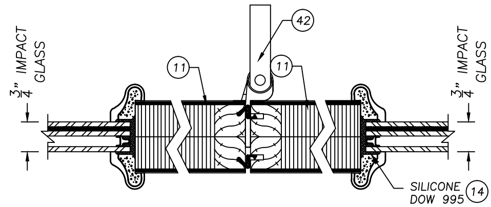
② HORIZONTAL CROSS SECTION ⑤ MIDDLE OF DOOR. VIEWED FROM TOP RAIL HALF OFFSET WITH HANDLE TO PULL INTERIOR SIDE
