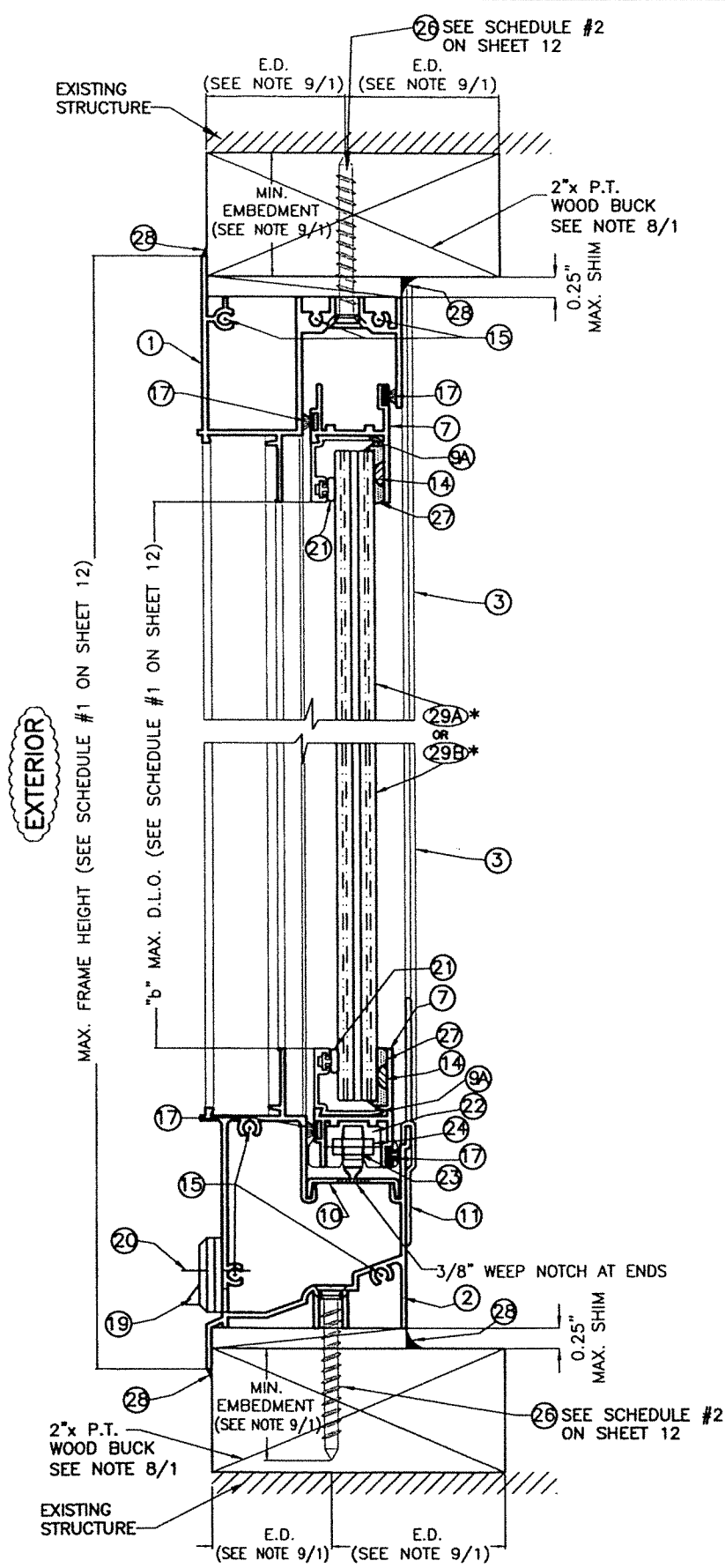
SECTION A-A (TO WOOD)
