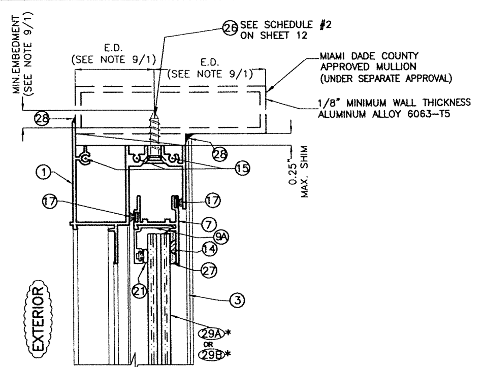
SECTION A-A (TO ALUMINUM MULLION)
