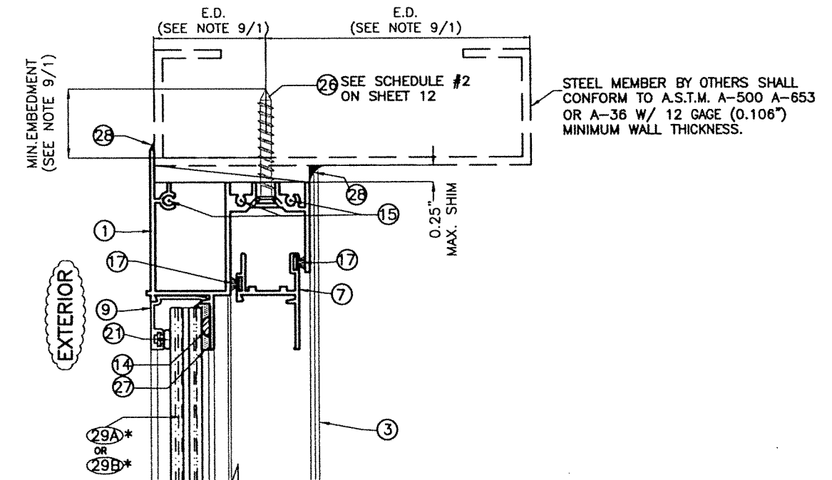
SECTION B-B (TO STEEL MEMBER)
