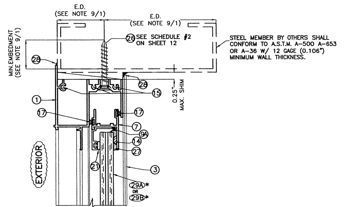
SECTION A-A (TO STEEL MEMBER)
