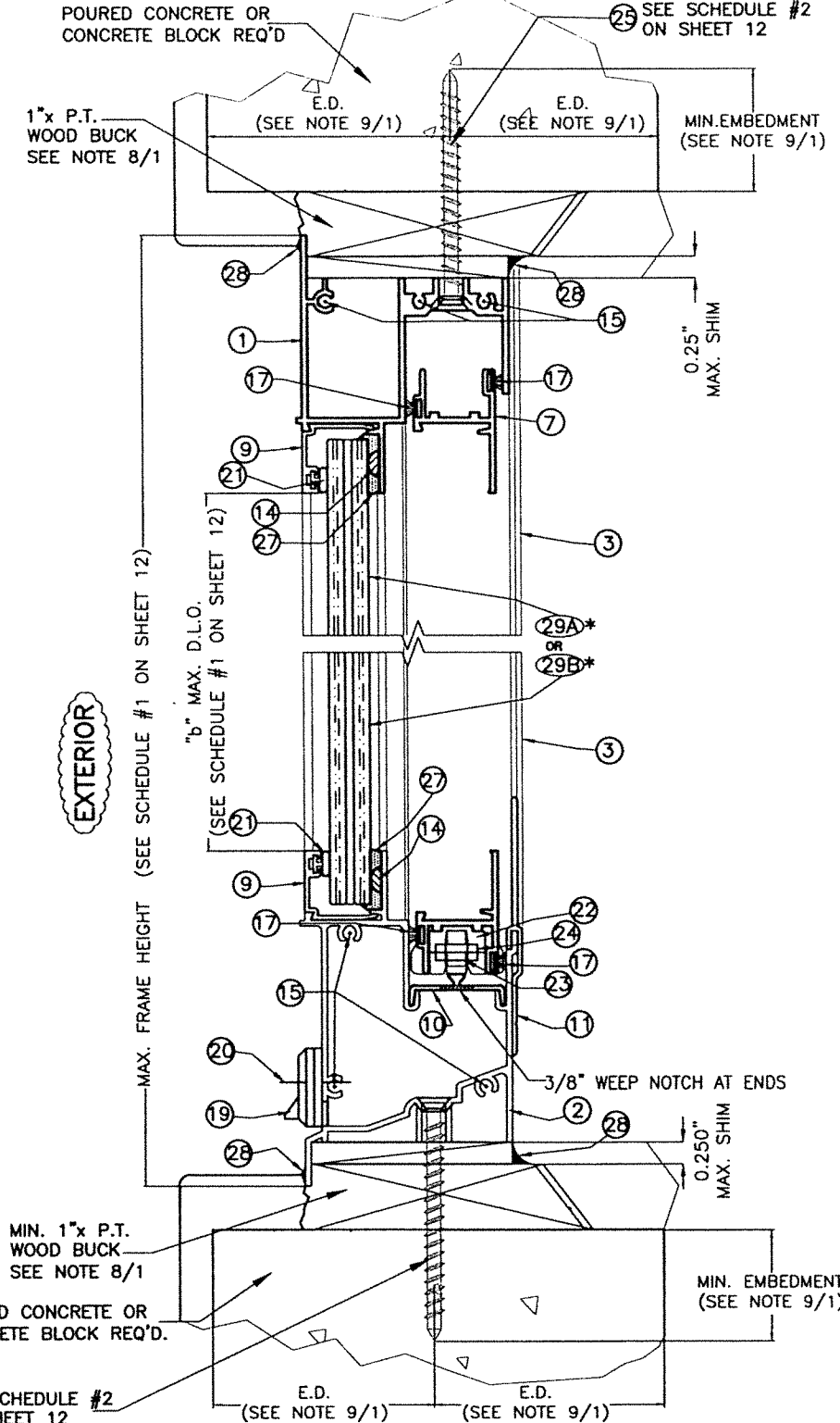
SECTION B-B (TO POURED CONCRETE OR CONCRETE BLOCK)
