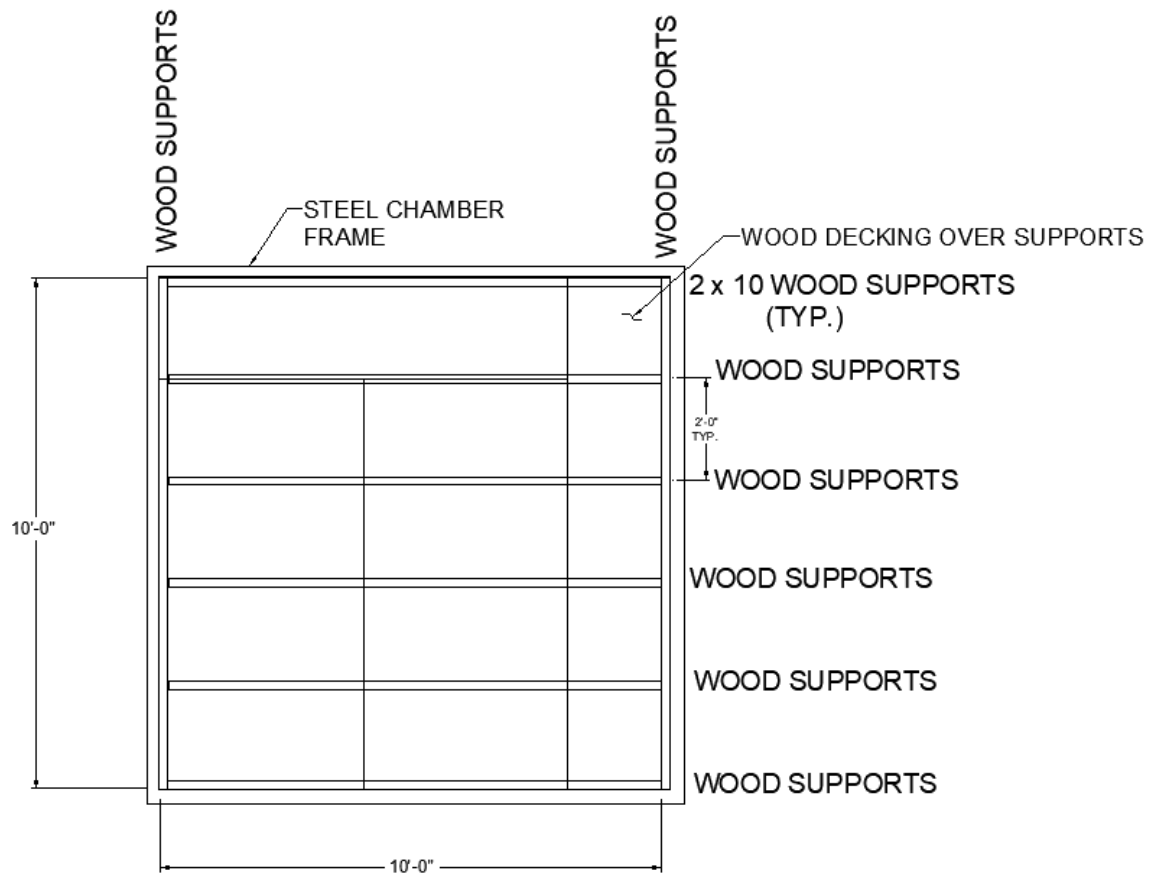
PLAN VIEW OF WOOD DECKING & SUPPORTS
