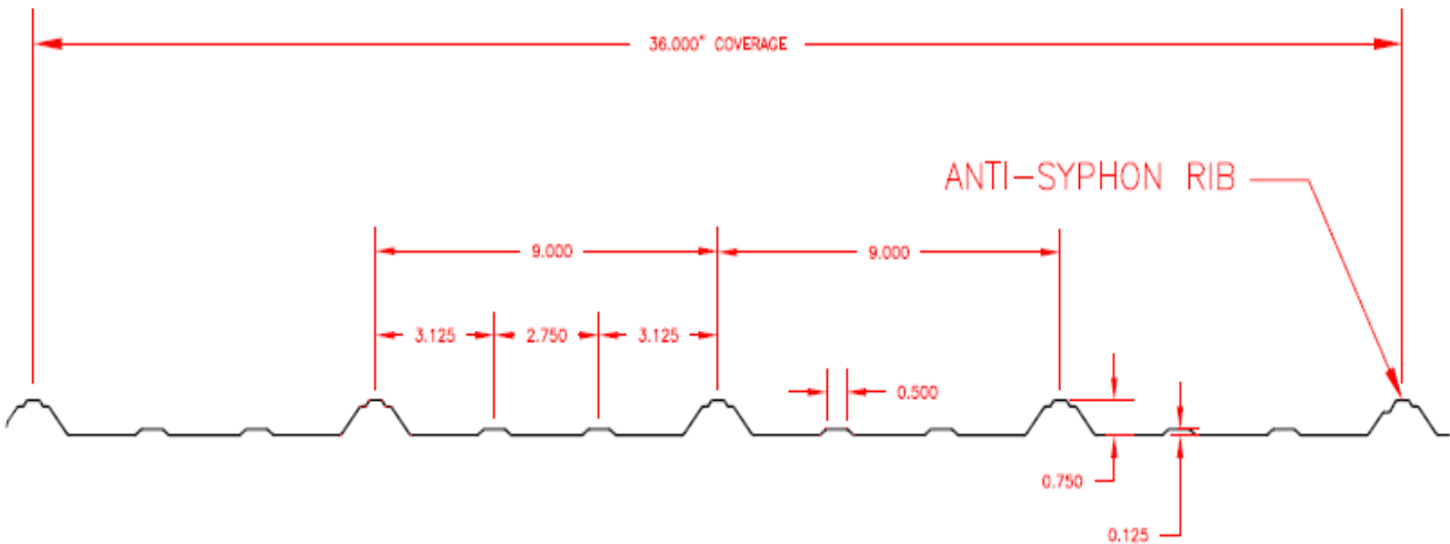
PANEL DETAIL
