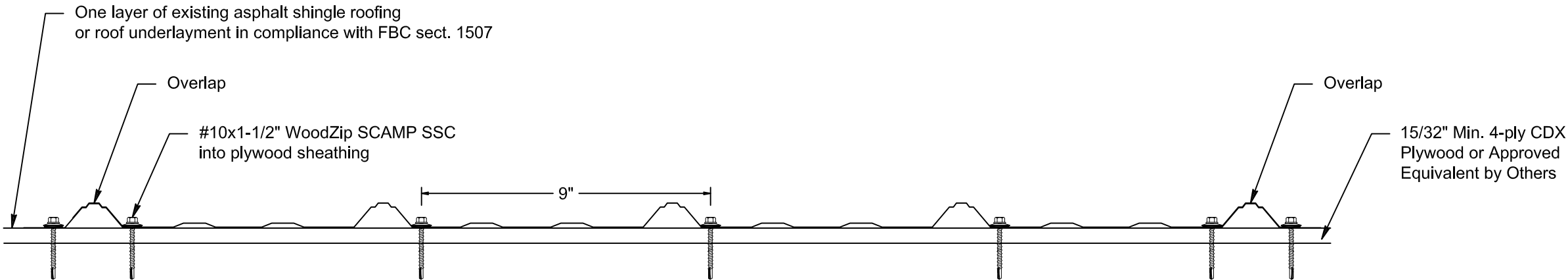
Fastener Pattern at Panel Ends (Eave/Ridge) and 24" O.C. in Field
