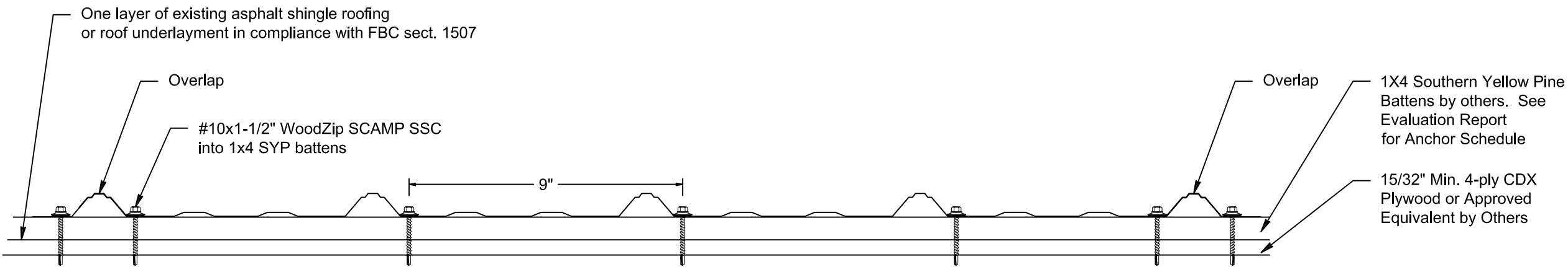
Fastener Pattern at Panel Ends (Eave/Ridge) and 24" O.C. in Field
