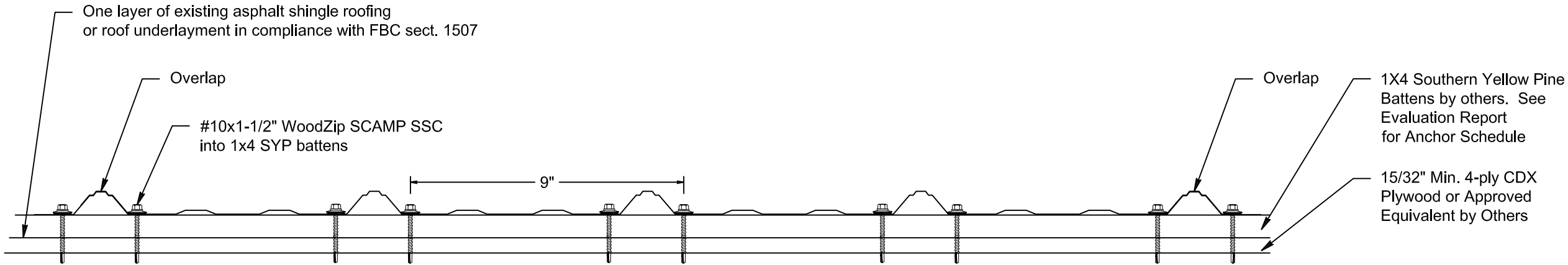
Fastener Pattern at Panel Ends (Eave/Ridge) and 24" O.C. in Field
