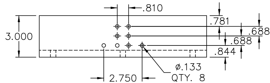
(164) 3xXx1/2" STEEL MULL CLIP FOR ATTACHMENT TO MOUNTING ANGLE
