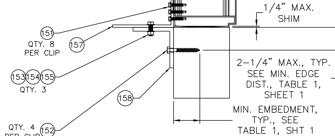
3x6x1/4" ALUMINUM MULL CLIP HEAD/SILL OPTIONAL ATTACHMENT TO 6" WALL WITH 4X4X3/8" ALUMINUM MOUNTING ANGLE
