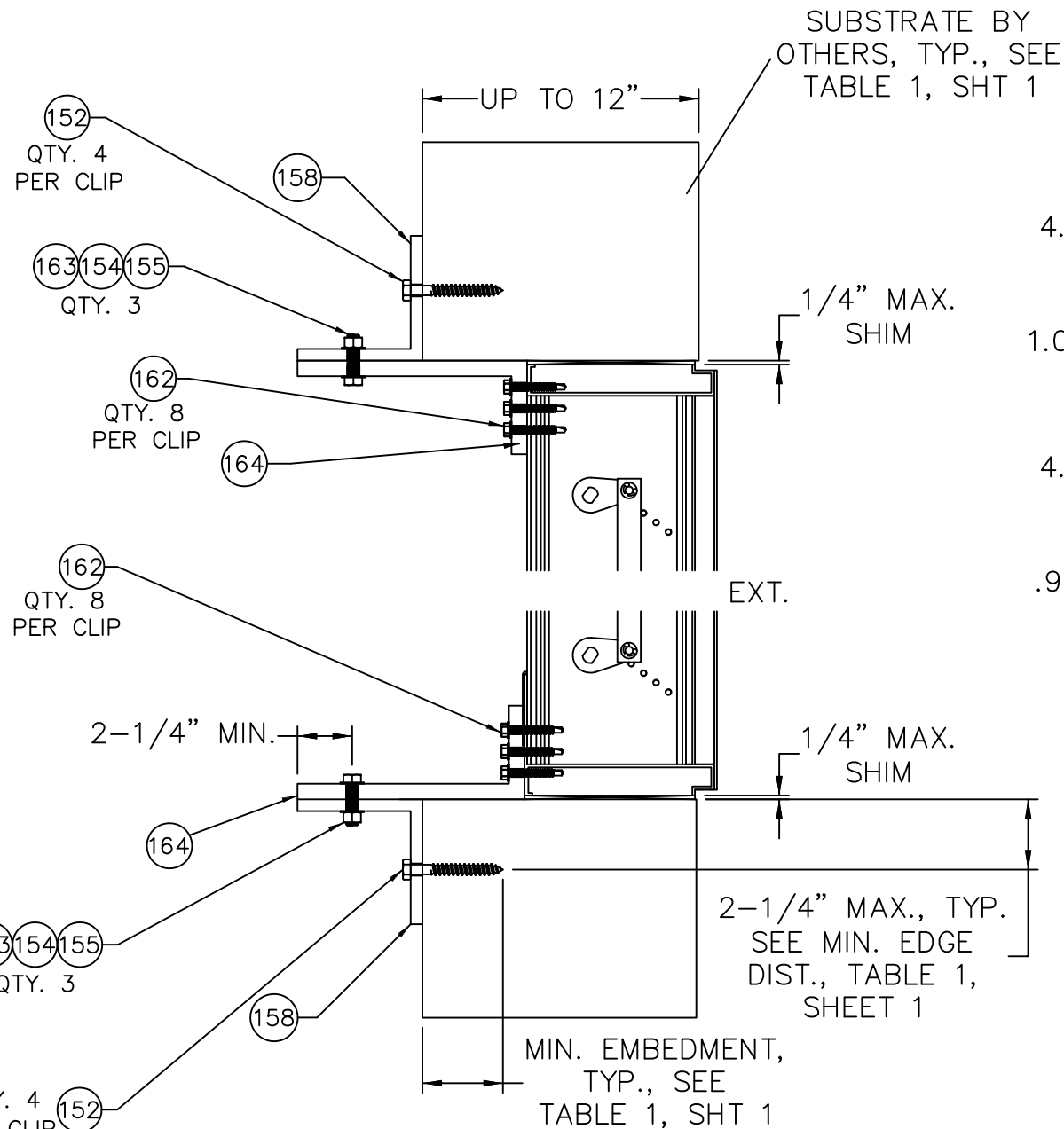
3xXx1/2" STEEL MULL CLIP HEAD/SILL OPTIONAL ATTACHMENT TO UP TO 12" WALL WITH 4x4x3/8" ALUMINUM MOUNTING ANGLE
