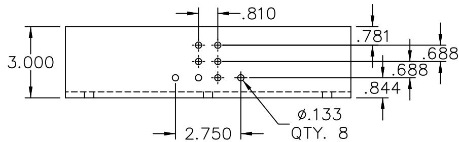
(157) 3x6x1/4" ALUMINUM MULL CLIP FOR ATTACHMENT TO MOUNTING ANGLE, 6" WALL
