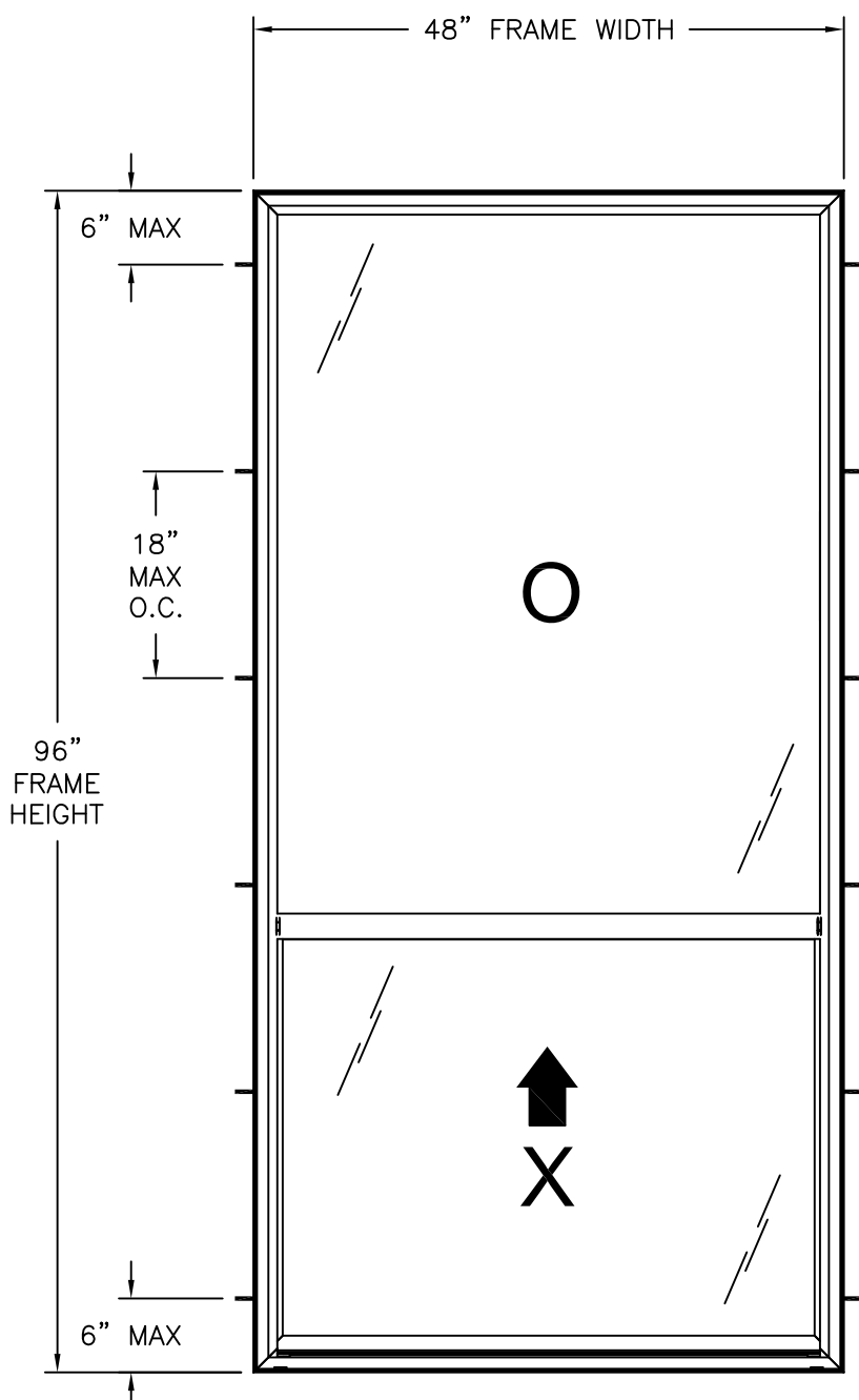
SERIES 3540 PVC SH WINDOW FRAME INSTALLATION EXTERIOR VIEW
