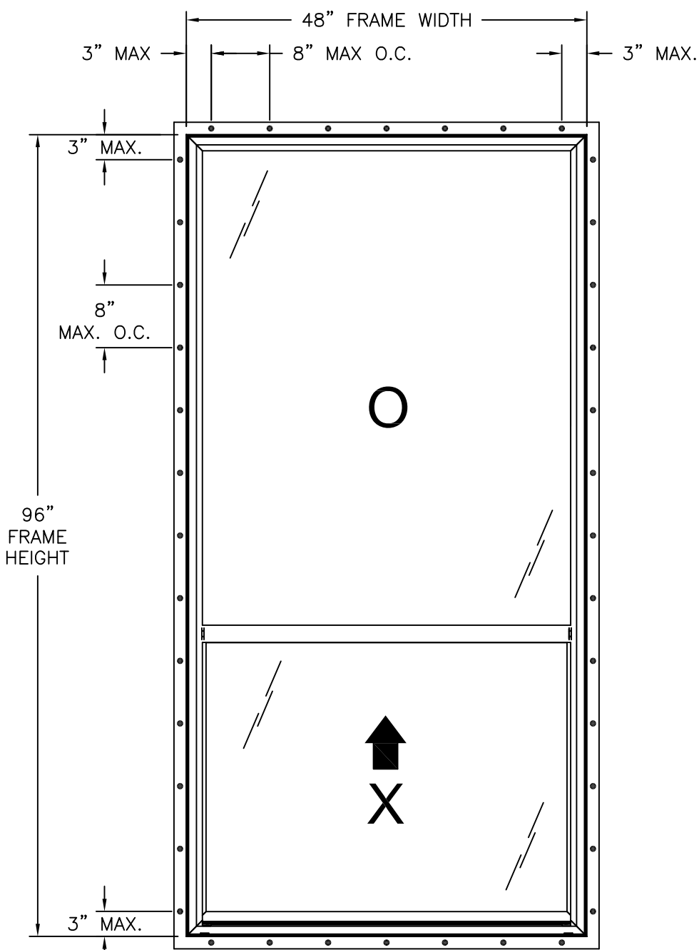
SERIES 3540 PVC SH WINDOW FIN INSTALLATION EXTERIOR VIEW
