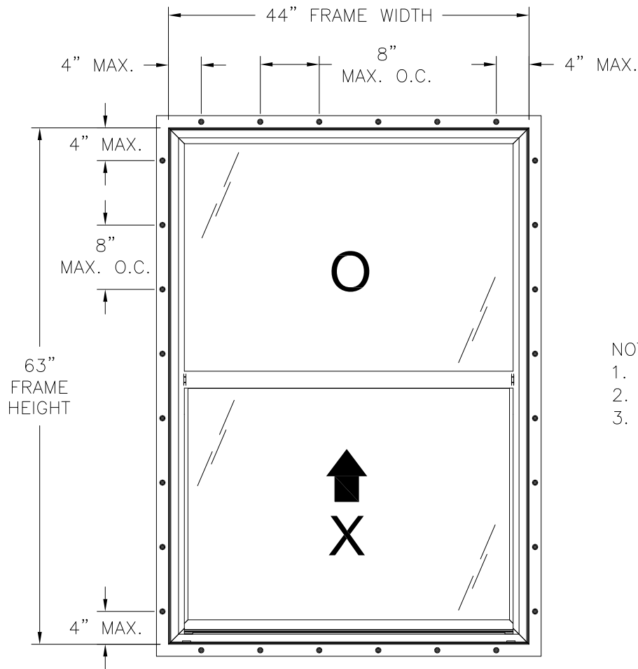
SERIES 3540 PVC SINGLE HUNG WINDOW EXTERIOR VIEW
