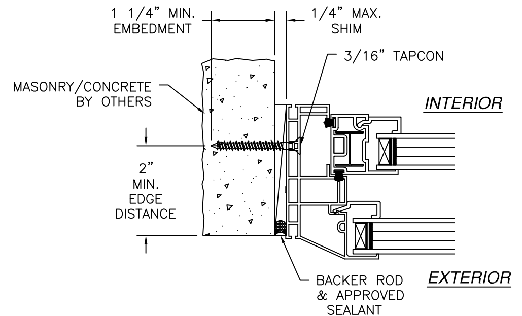
HORIZONTAL INSTALLATION DETAIL CONCRETE/MASONRY WITHOUT 1X BUCK INSTALLATION FOR CONCRETE/MASONRY WITH 1X BUCK REFER TO HEAD AND SILL INSTALLATION DETAILS
