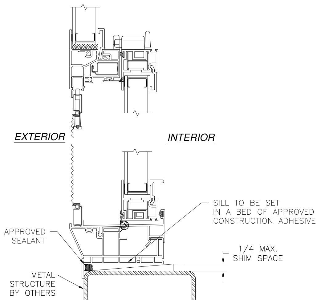
VERTICAL CROSS SECTION METAL STRUCTURE INSTALLATION
