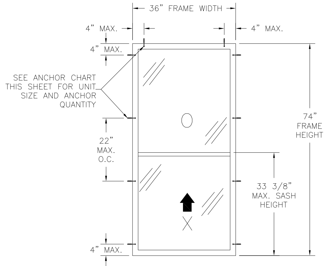
SERIES 3540 FLANGE PVC SINGLE HUNG WINDOW EXTERIOR VIEW
