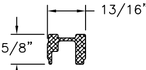
REINFORCEMENT (15953) ALUMINUM 6063-T5
