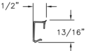
GLAZING BEAD (856) EXTRUDED PVC
