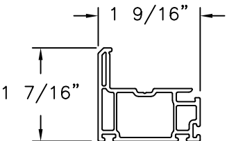
STILE (1808) EXTRUDED PVC
