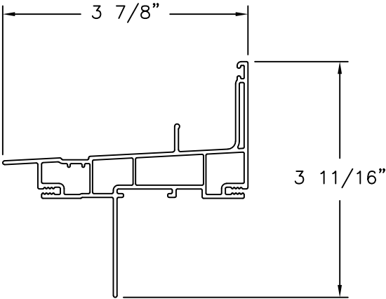
SILL (1852) EXTRUDED PVC
