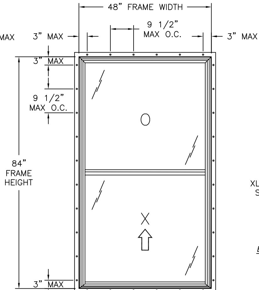
G110 PVC SINGLE HUNG WINDOW FIN INSTALLATION
