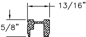
REINFORCEMENT (15953) ALUMINUM 6063-T5
