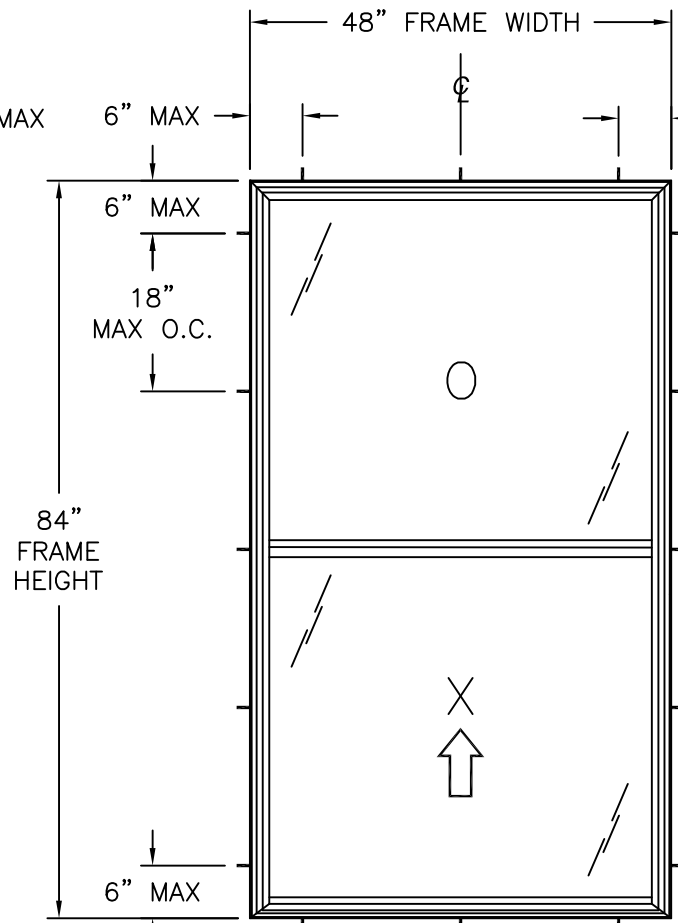
G110 PVC SINGLE HUNG WINDOW STRAP INSTALLATION
