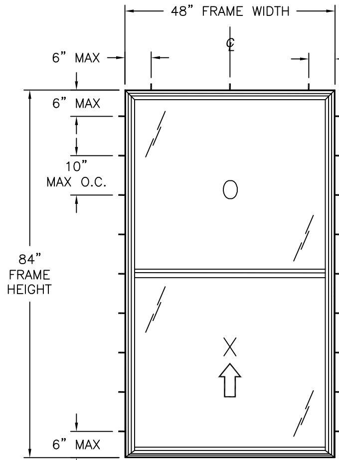
G110 PVC SINGLE HUNG WINDOW FINLESS INSTALLATION
