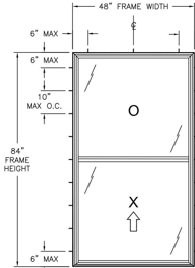
G110 PVC SINGLE HUNG WINDOW FINLESS INSTALLATION
