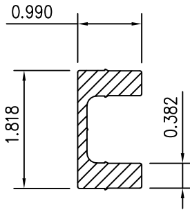
PANIC BAR ALUMINUM INSERT
