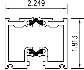
18 FRAME NARROW
