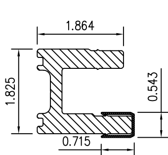
21 REGULAR RAIL INSERT
