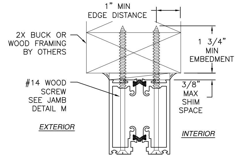
JAMB INSTALLATION DETAIL 2X BUCK OR WOOD FRAMING S45004 NO REINFORCEMENT
