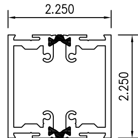
42 MULLION FRAME
