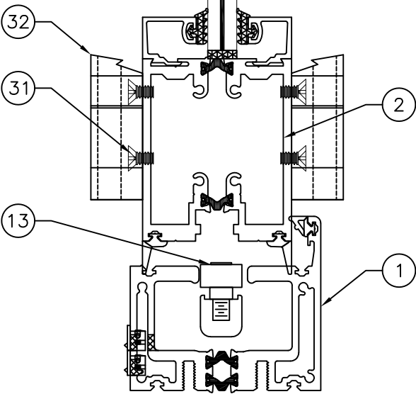
F 6 VERTICAL CROSS SECTION TOP LOAD
