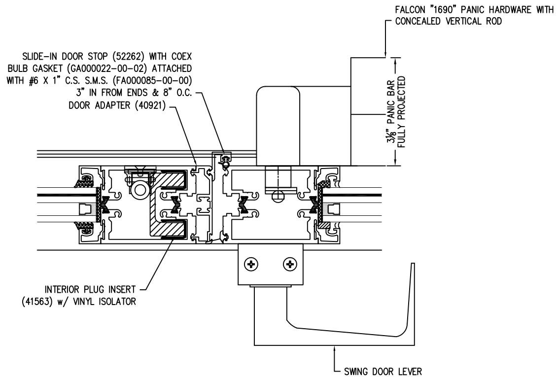
PANIC BAR DETAILS
