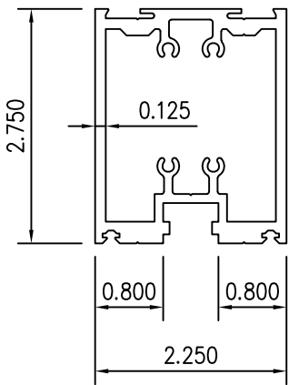
10 FRAME NON-THERMAL
