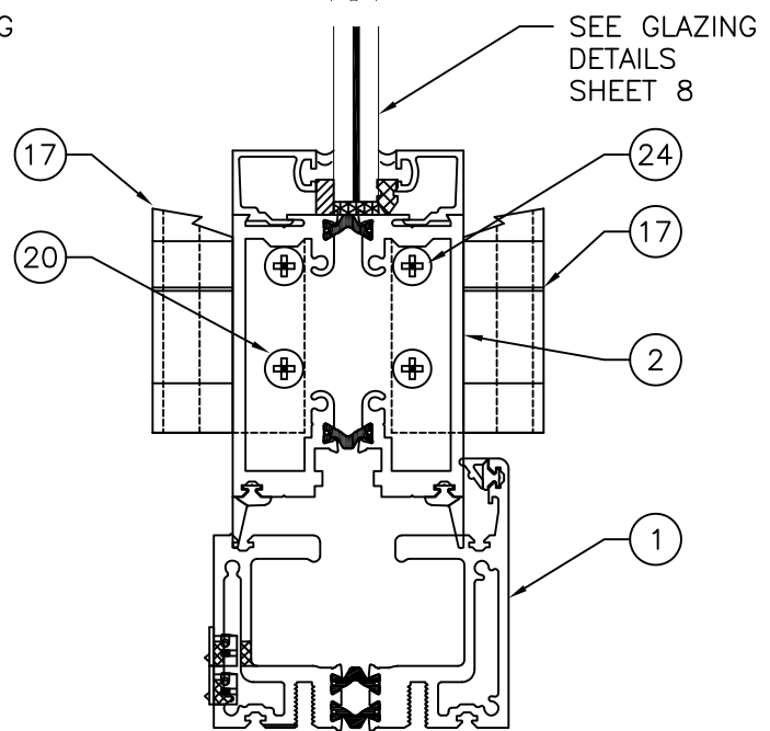
B 5 VERTICAL CROSS SECTION
