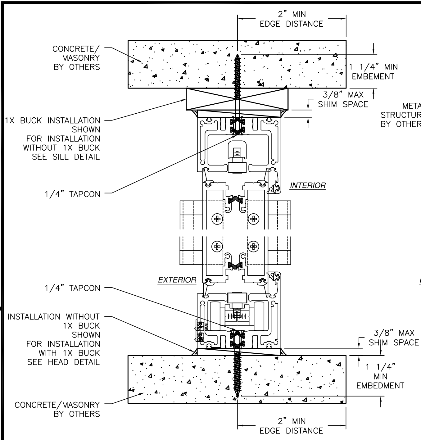
VERTICAL CROSS SECTION CONCRETE/MASONRY INSTALLATION STANDARD SILL SHOWN FLUSH SILL SIMILAR
