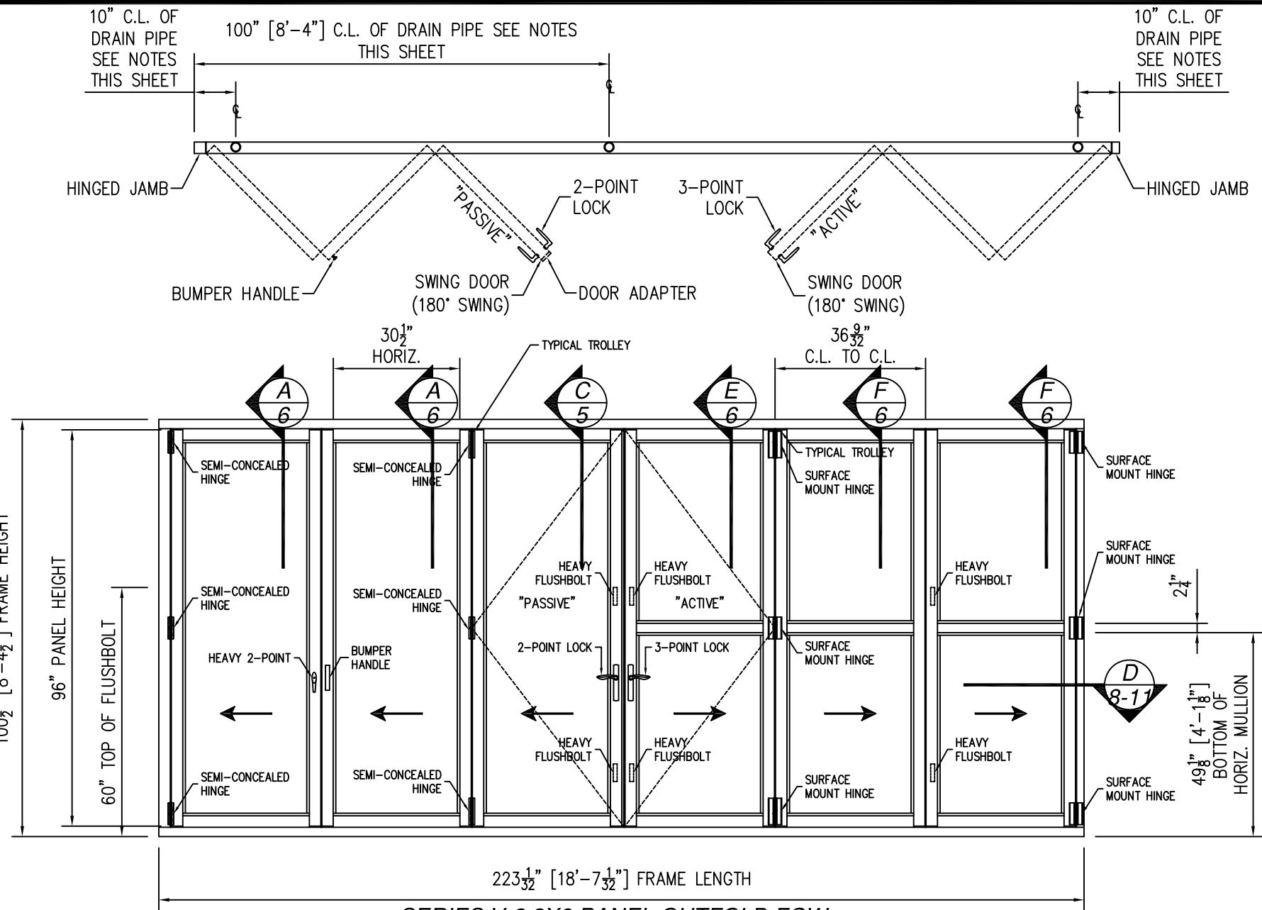
SERIES V-2 3X8 PANEL OUTFOLD FGW
