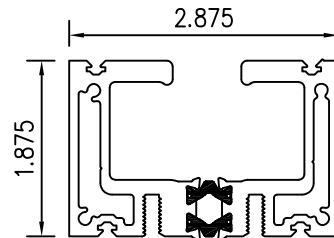
16 FLUSH SILL
