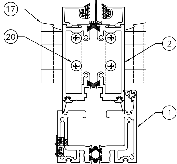
E 6 VERTICAL CROSS SECTION
