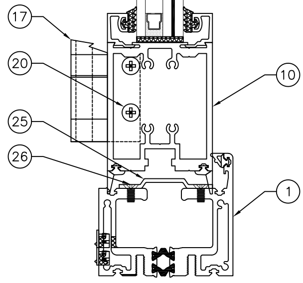
A 6 VERTICAL CROSS SECTION NON-THERMAL PANEL
