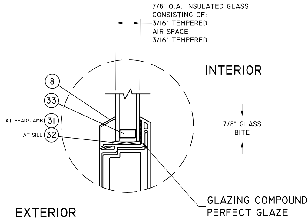
GLAZING DETAIL 2
