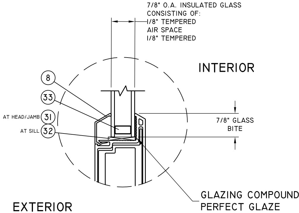
GLAZING DETAIL 1
