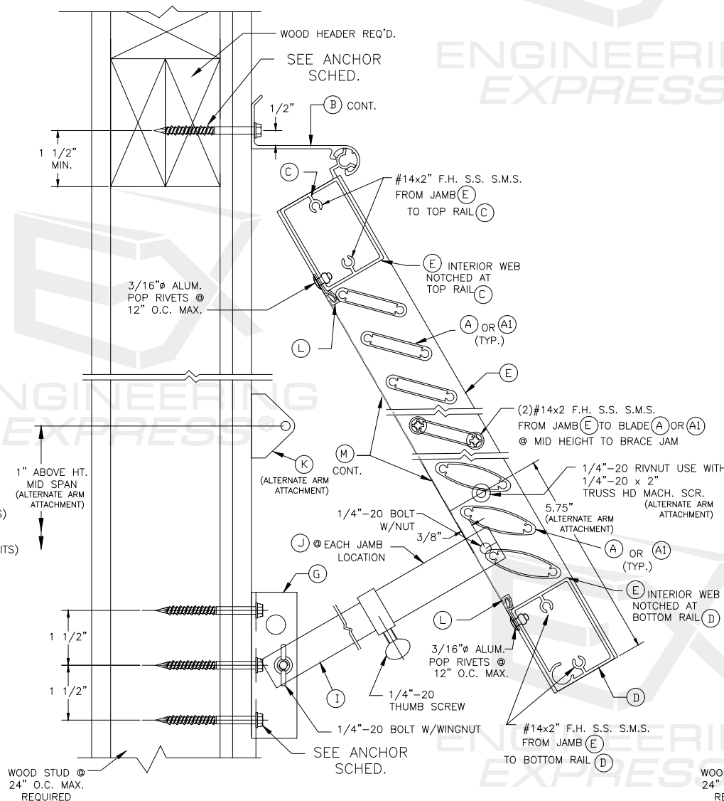
SECTION D (WALL MOUNT) NON-HURRICANE POSITION
