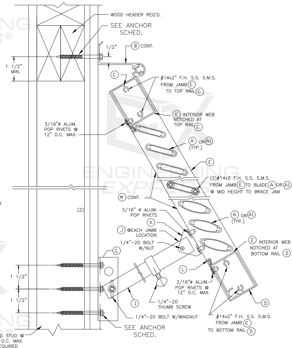
SECTION D* (WALL MOUNT) NON-HURRICANE POSITION
