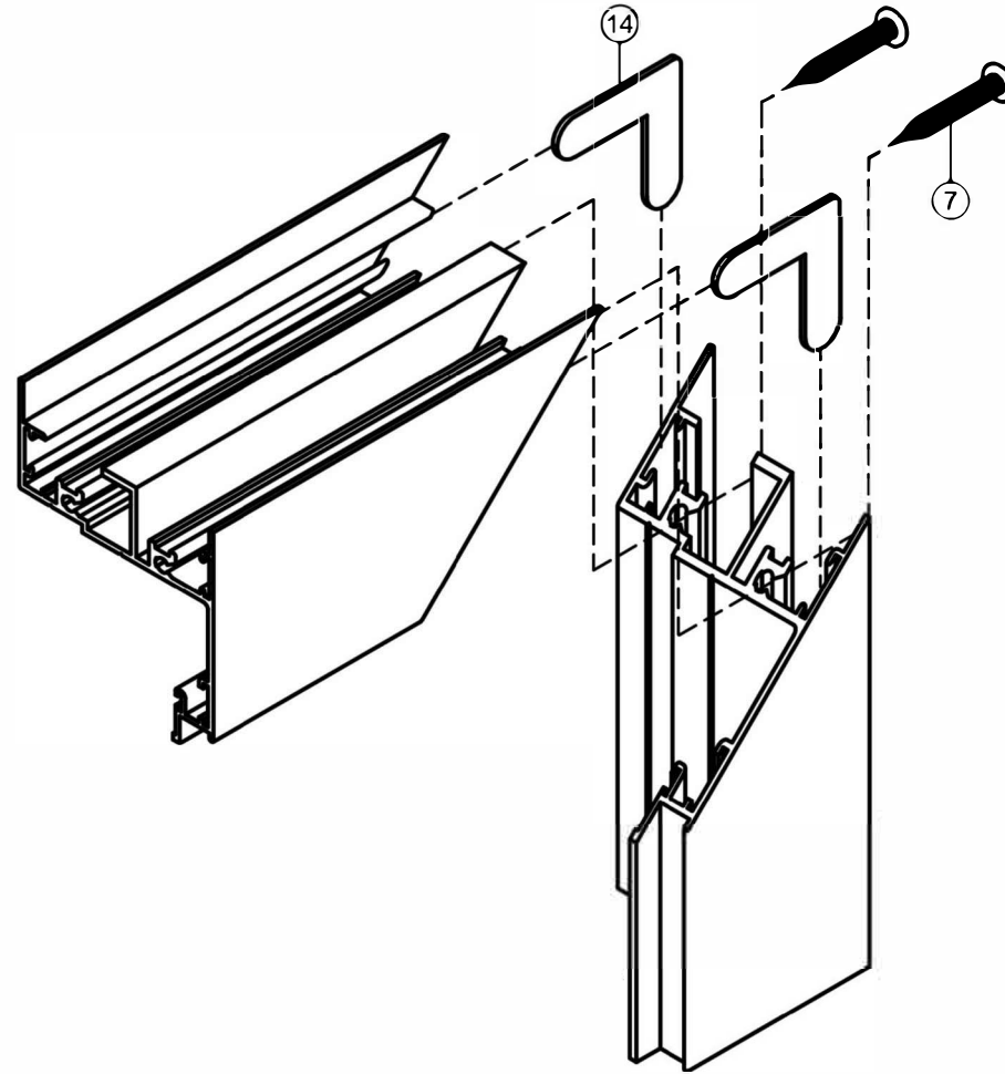
FRAME CORNERS
