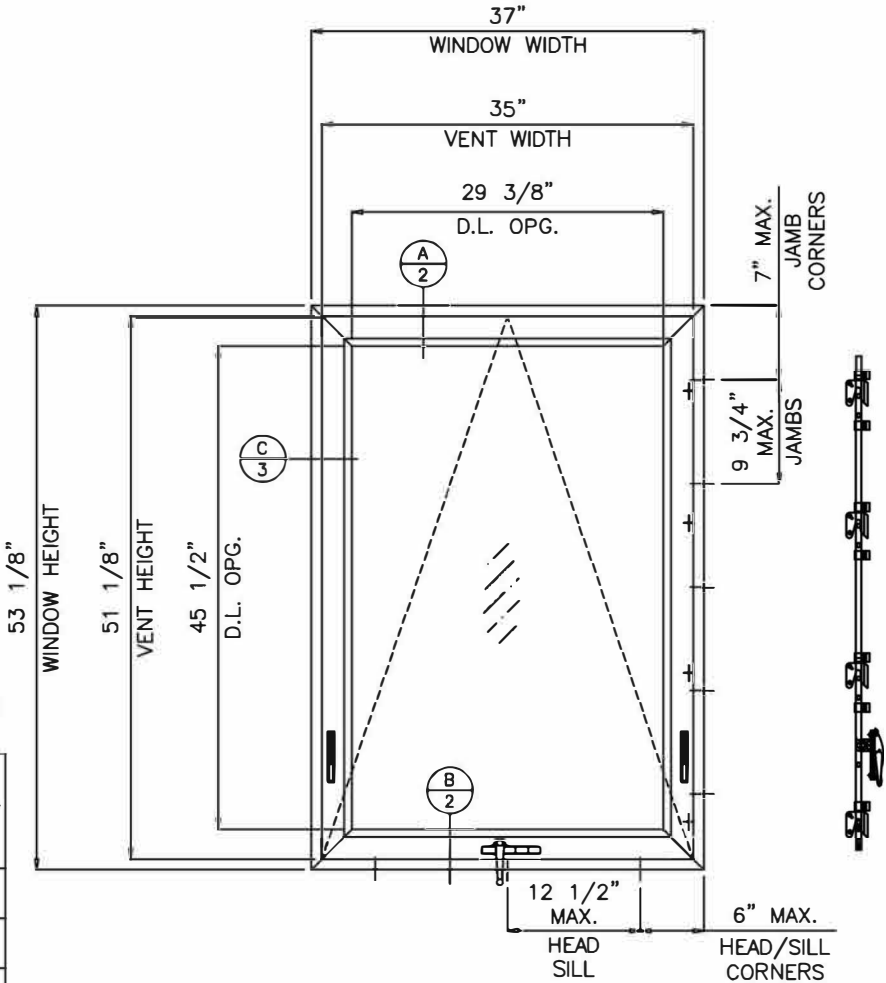
TYPICAL ELEVATION
