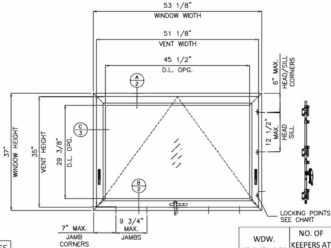
TYPICAL ELEVATION
