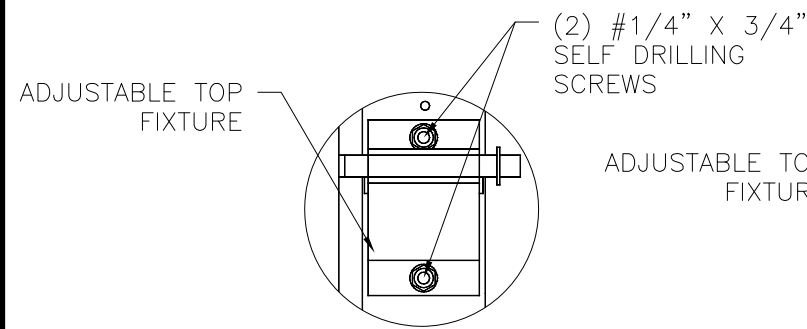
DETAIL A TOP FIXTURE
