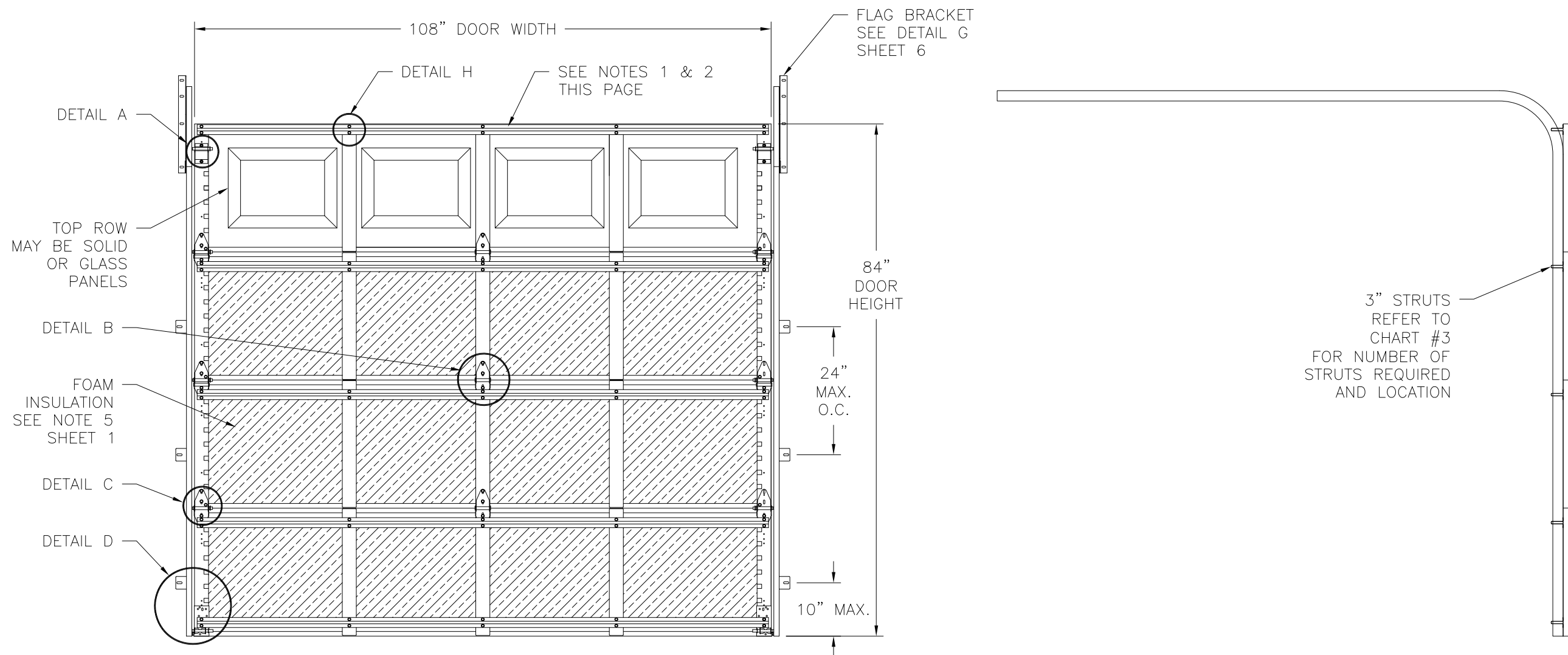
140C CHOICE SERIES GARAGE DOOR OPAQUE SHOWN, GLAZED SIMILAR INTERIOR VIEW FOR RATINGS, NUMBER OF JAMB BRACKETS AND STRUTS REQUIRED SEE SHEET 3
