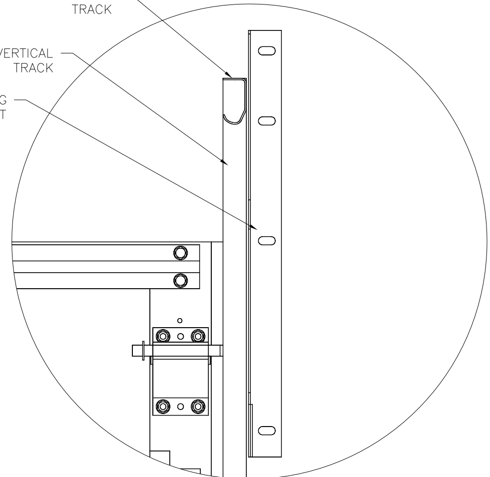
DETAIL G FLAG BRACKET
