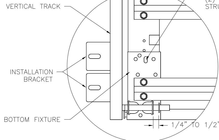
DETAIL F BOTTOM FIXTURE
