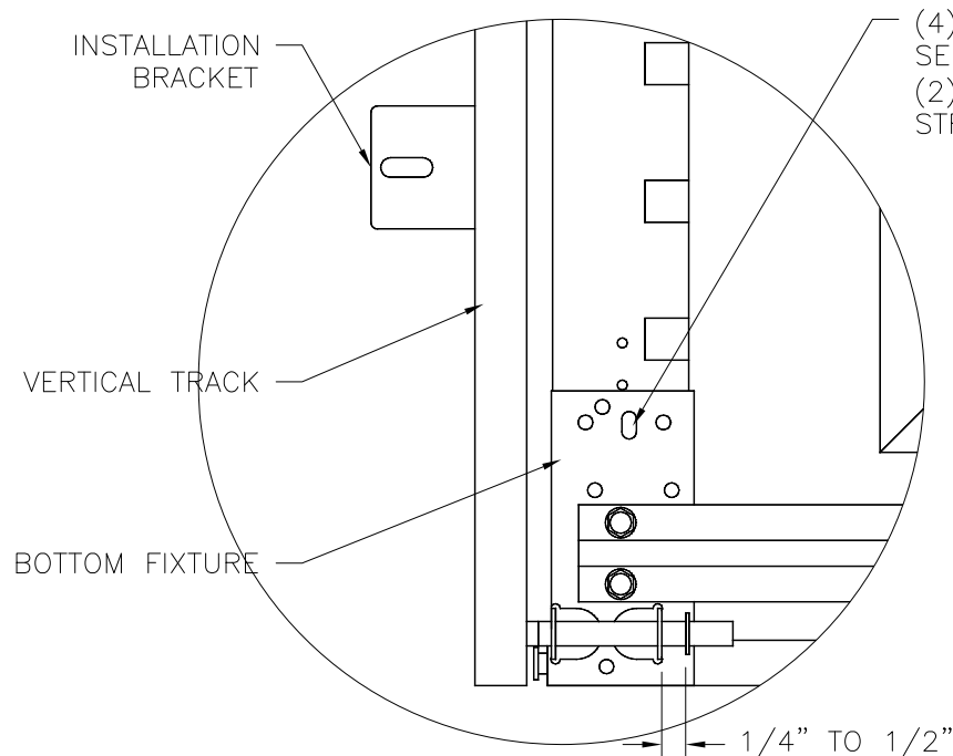
DETAIL D BOTTOM FIXTURE
