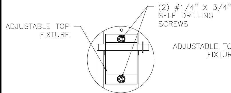
DETAIL A TOP FIXTURE
