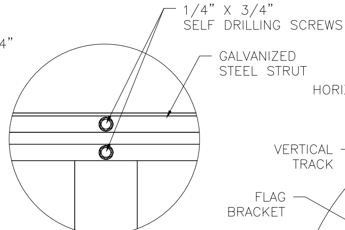
DETAIL H STEEL STRUT
