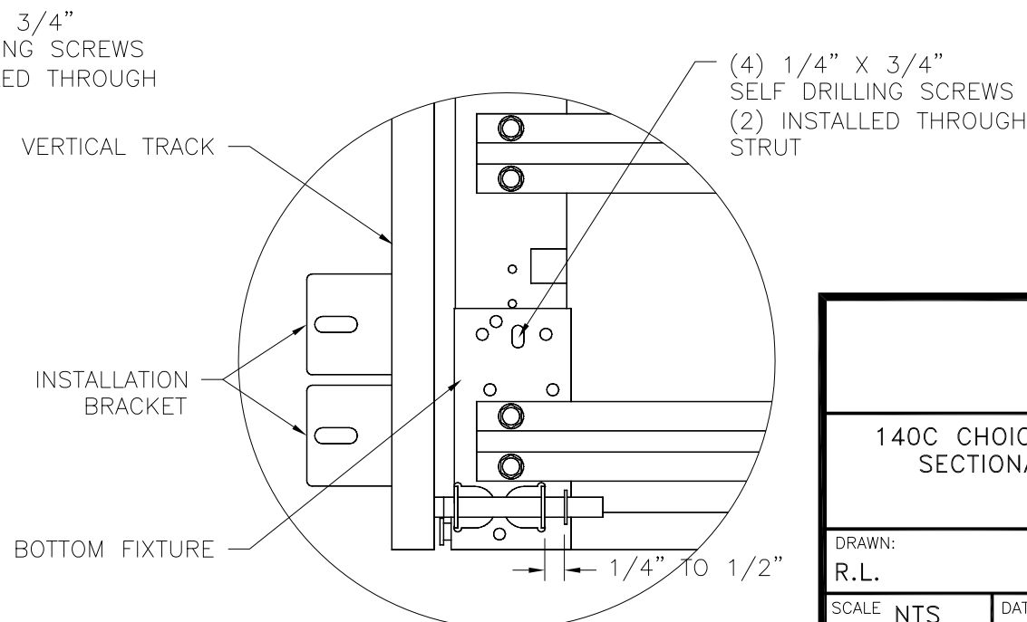
DETAIL F BOTTOM FIXTURE
