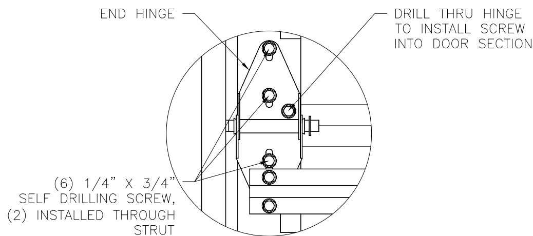
DETAIL C END HINGE
