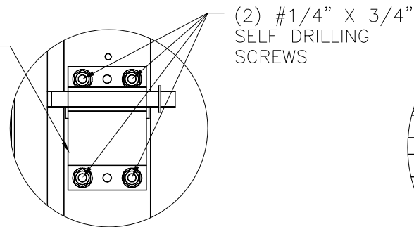
DETAIL E TOP FIXTURE
