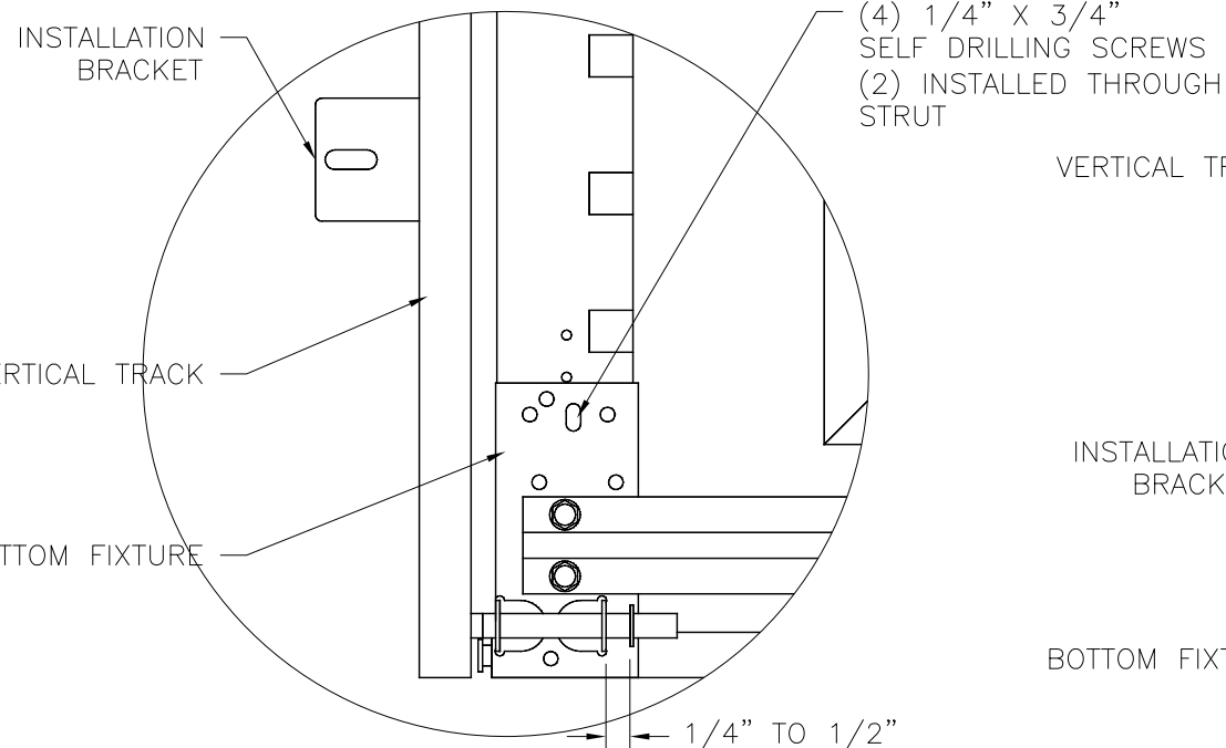
DETAIL D BOTTOM FIXTURE
