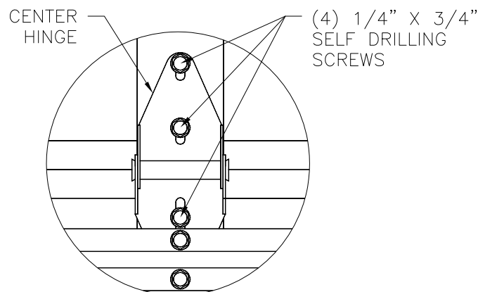
DETAIL B CENTER HINGE
