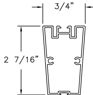
MULLION ALUMINUM
