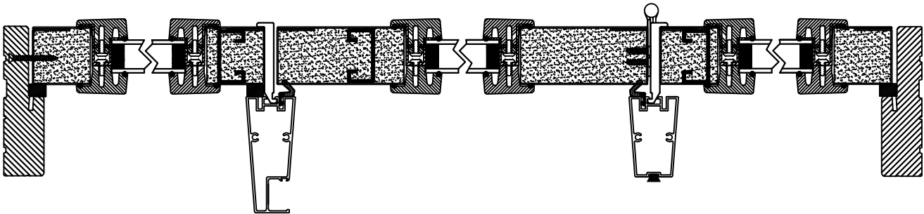
HORIZONTAL CROSS SECTION
