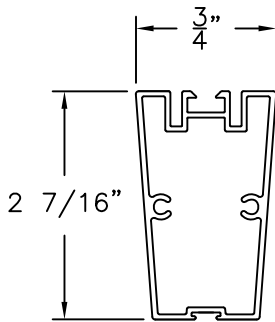
MULLION ALUMINUM
