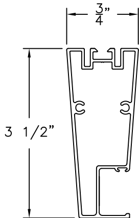
MULLION ALUMINUM
