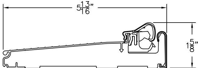
ENDURA ZAC THRESHOLD W/ ARTICULATING CAP
