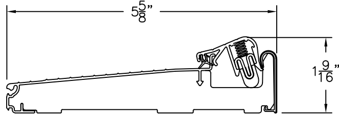
ZAC THRESHOLD W/ ARTICULATING CAP
