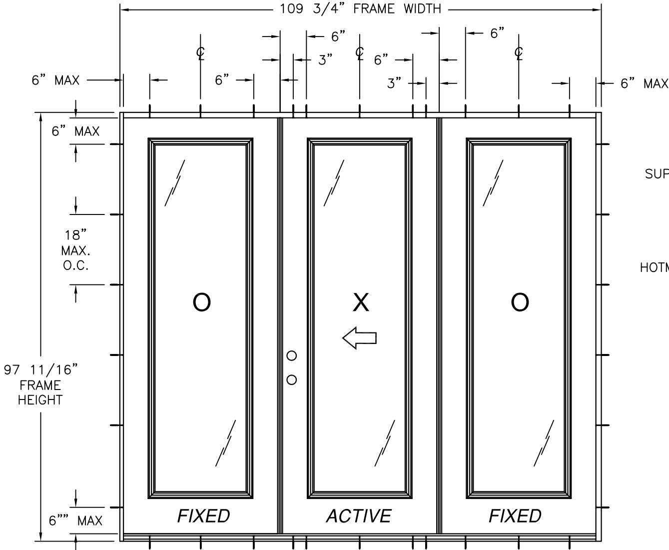
FIBERGLASS PATIO DOOR OXO EXTERIOR VIEW
