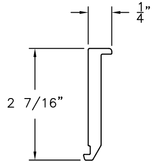
MULLION SPACER PVC
