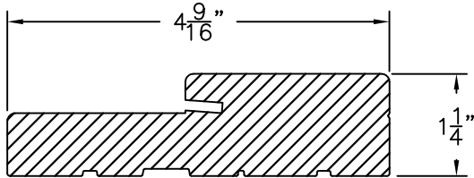
FRAMESAVER COMPOSITE
