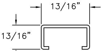
TOP C CHANNEL WOOD G.46 MIN.
