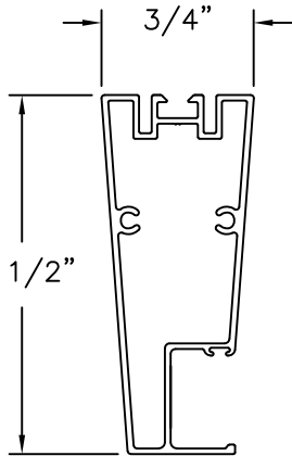
MULLION ALUMINUM
