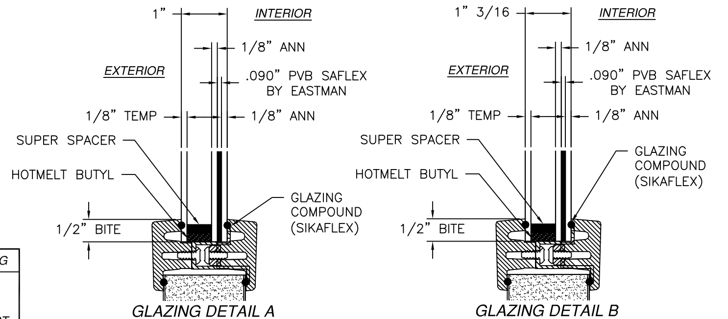
HORIZONTAL CROSS SECTION
