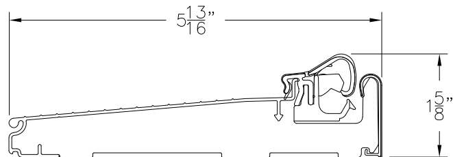
ENDURA ZAC THRESHOLD W/ ARTICULATING CAP
