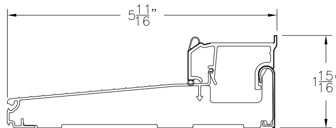
ZAC THRESHOLD W/90 SERIES I/S SIDELITE SILL CAP
