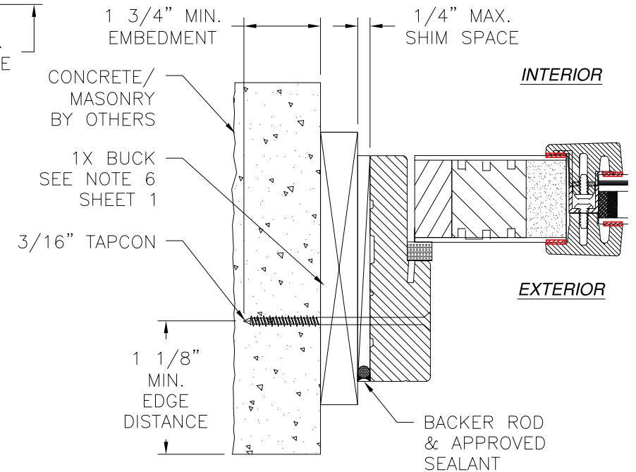
JAMB INSTALLATION DETAIL CONCRETE/MASONRY INSTALLATION
