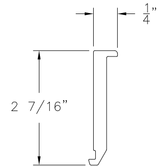
MULLION SPACER PVC
