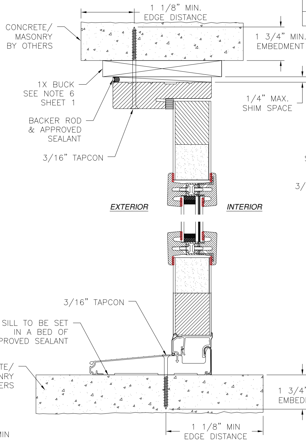
VERTICAL CROSS SECTION SIDELITE INSTALLATION CONCRETE/MASONRY INSTALLATION
