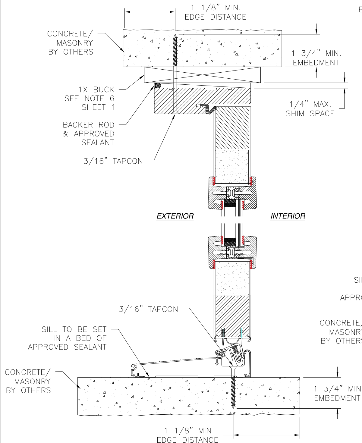
VERTICAL CROSS SECTION DOOR INSTALLATION CONCRETE/MASONRY INSTALLATION
