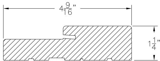
FRAMESAVER COMPOSITE
