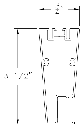
MULLION ALUMINUM
