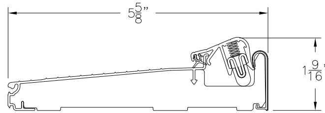
ZAC THRESHOLD W/ ARTICULATING CAP
