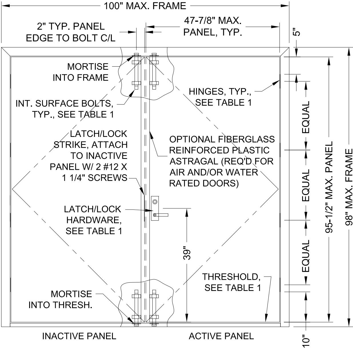
OUTSWING PAIR ELEVATION
