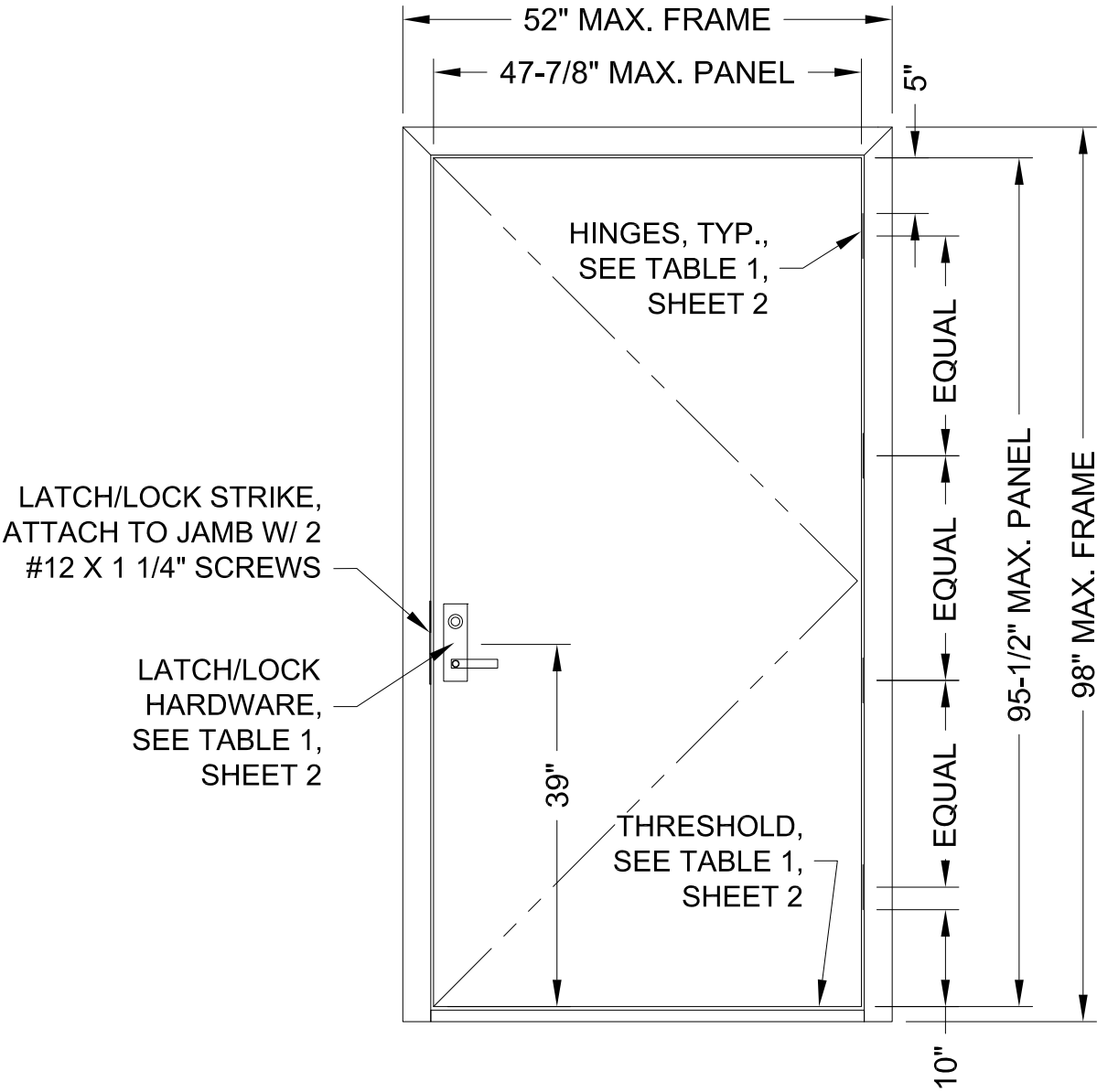
OUTSWING SINGLE ELEVATION
