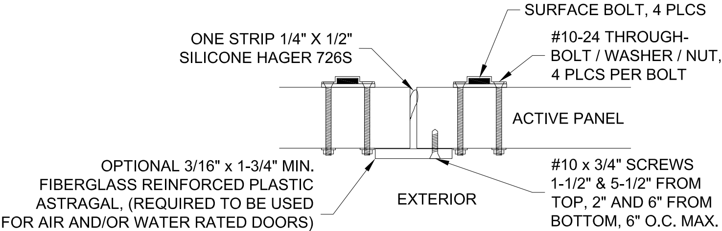
DOOR PAIR MEETING STILES DETAIL
