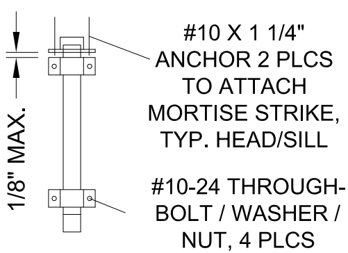
TYP. SURFACE BOLT ANCHORAGE
