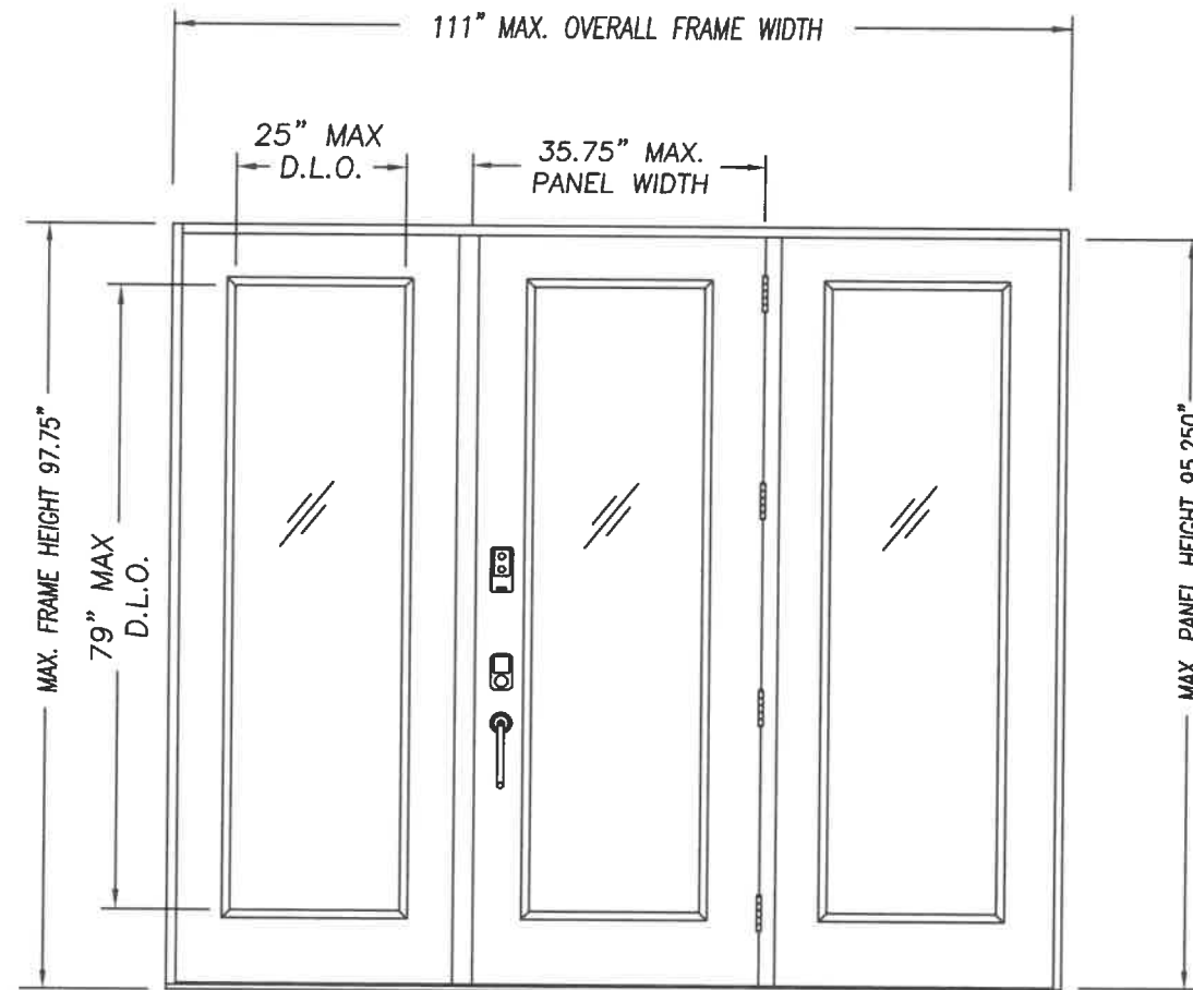
SINGLE DOOR UNIT W/SIDELITES
