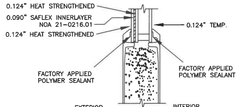
EXTERIOR INTERIOR TYPICAL GLAZING DETAIL IMPACT RATED GLASS
