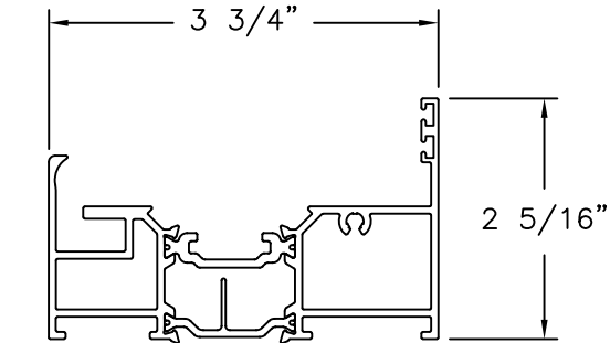
LATERAL FRAME (S85HJAMB) ALUMINUM 6063-T5
