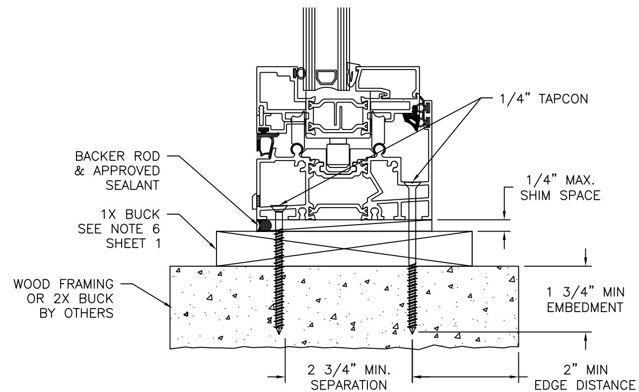
VERTICAL CROSS SECTION CONCRETE/MASONRY W/1X BUCK INSTALLATION
