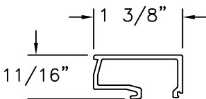
GLAZING STOP (S85GLHV) ALUMINUM 6063-T5
