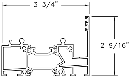
SILL / BOTTOM TRACK (S850SS1LL) ALUMINUM 6063-T5
