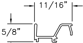
PULL HANDLE (S85GLV) ALUMINUM 6063-T5
