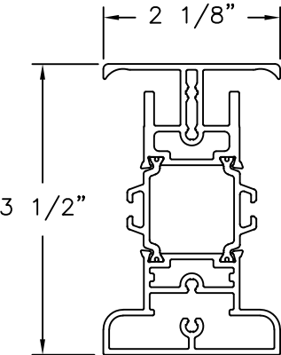
POST / REINFORCEMENT MULLION (S85POST) ALUMINUM 6063-T5
