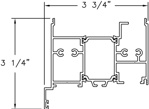
PANEL JAMB EXTENDER (S85JAMBEXT) ALUMINUM 6063-T5
