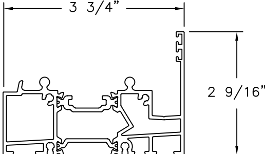
SILL TRACK (S850SS1LLDU) ALUMINUM 6063-T5
