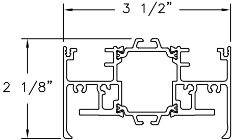
POST W/ROLLER (S85EVEN_ROLLER) ALUMINUM 6063-T5
