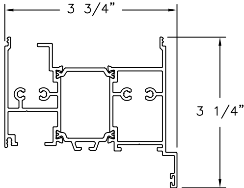
PANEL JAMB EXTENDER (S85JAMBEXT) ALUMINUM 6063-T5
