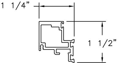
PANEL (S85PANEL) ALUMINUM 6063-T5
