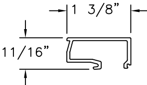
GLAZING STOP (S85GLHV) ALUMINUM 6063-T5
