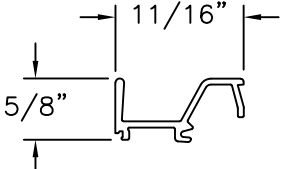
PULL HANDLE (S85GLV) ALUMINUM 6063-T5
