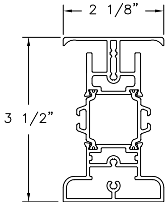
CONCEALED HINGE(S85H1NGE) ALUMINUM 6063-T5
