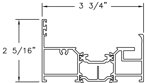
LATERAL FRAME (S85HJAMBDU) ALUMINUM 6063-T5
