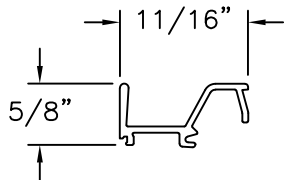
GLAZING STOP (S85GLV) ALUMINUM 6063-T5
