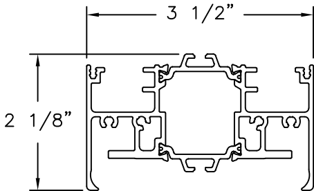
POST W/ROLLER (S85EVEN_ROLLER) ALUMINUM 6063-T5
