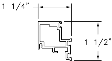
PANEL (S85PANELDU) ALUMINUM 6063-T5
