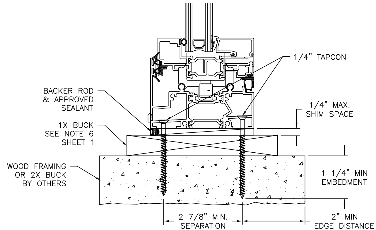
VERTICAL CROSS SECTION CONCRETE/MASONRY W/1X BUCK INSTALLATION
