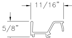
PULL HANDLE (S85GLV) ALUMINUM 6063-T5
