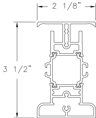
POST / REINFORCEMENT MULLION (S85POST) ALUMINUM 6063-T5
