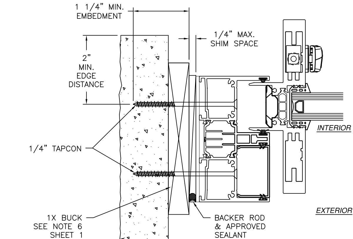
JAMB INSTALLATION DETAIL CONCRETE/MASONRY W/1X BUCK INSTALLATION
