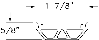
SMALL SPACER (S100SPACERS) PVC
