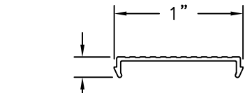
SILL SNAP FILLER (S100SNAP) ALUMINUM 6063-T5
