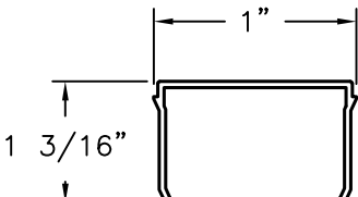
FINGER GASKET (S100G1F) ALUMINUM 6063-T5
