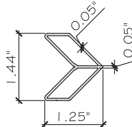
12 CORNER KEY ES-45T-011 ALUM.6063-T5
