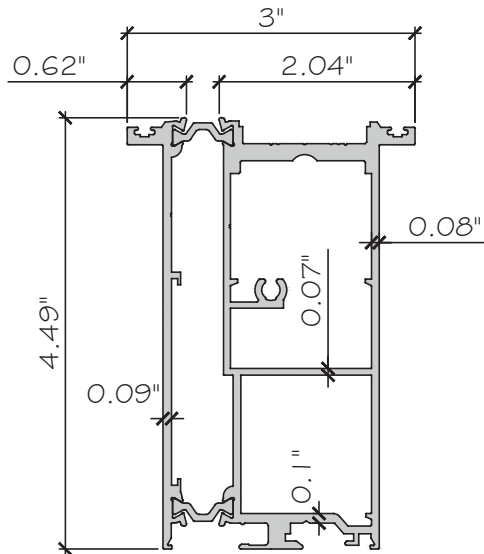
4 LEAF TOP 029 FRONT + 008 BACK ES-PSD5030T-502 ALUM.6063-T6
