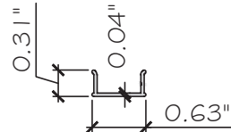
9 JAMB SCREW COVER ES-EL114 ALUM.6063-T6
