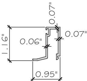
11 EXTERIOR GLASS STOP ES-PSD5030T-013 ALUM.6063-T5
