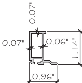
10 INTERIOR GLASS STOP ES-PSD5030T-014 ALUM.6063-T5
