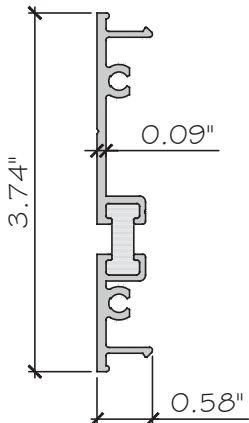
3 SHEAR CLIP ES-8000T-003T ALUM.6063-T6
