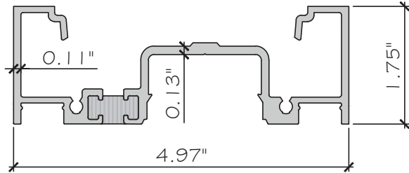
2 FRAME HEAD ES-PSD5030T-002T ALUM.6005-T5
