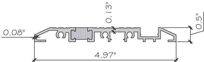
6 THRESHOLD ES-PSD5030T-005T ALUM.6063-T6
