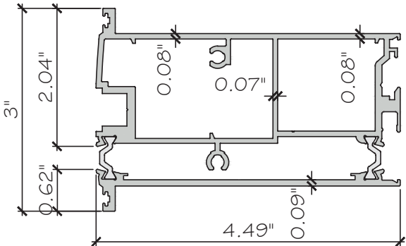
5 LEAF STILE 006 FRONT + 007 BACK ES-PSD5030T-501 ALUM.6063-T6
