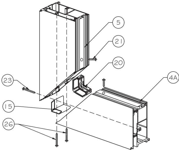
CORNER ASSEMBLY
