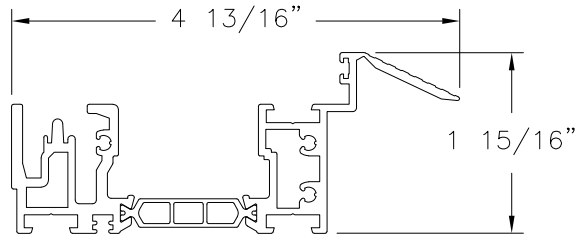
HYBRID SILL PROFILE (5-320-09) ALUMINUM 6063-T5
