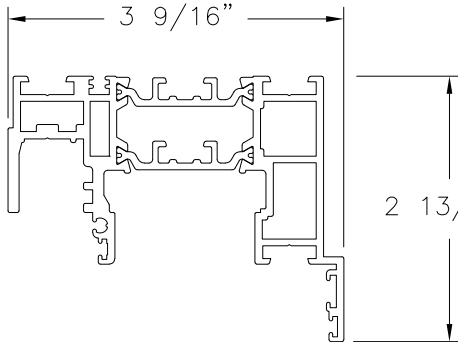
HEAD & JAMB PROFILE (5-320-04) ALUMINUM 6063-T5
