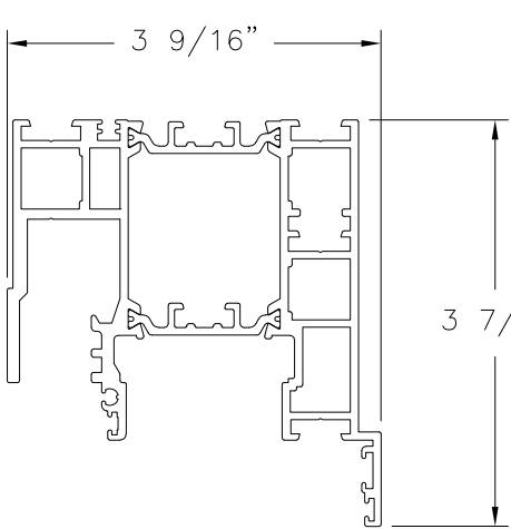
EXTENDED HEAD PROFILE ALUMINUM 6063-T5
