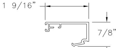
GLAZING BEAD (5-300-14) ALUMINUM 6063-T5 BEAD SHOWN AS REFERENCE ONLY. BEAD SIZES VARIES DEPENDING ON GLASS THICKNESS. GLASS THICKNESS VARIES FROM 3/16" TO 1 3/4"
