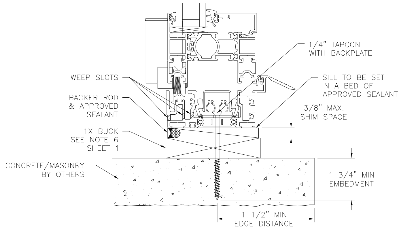
VERTICAL CROSS SECTION CONCRETE/MASONRY W/1X BUCK INSTALLATION HYBRID SILL SHOWN, OTHER SILLS SIMILAR
