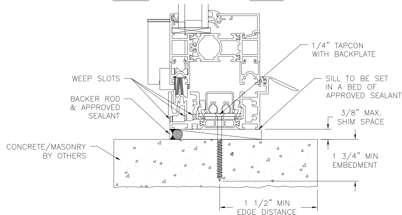
VERTICAL CROSS SECTION CONCRETE/MASONRY INSTALLATION HYBRID SILL SHOWN, OTHER SILLS SIMILAR
