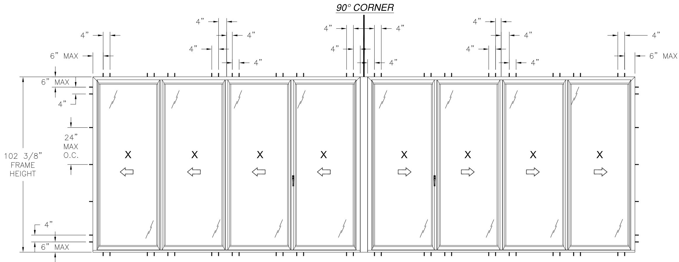
SERIES NW REINFORCED 847/SL84/HIGHLINE CORNER FOLDING PANEL SYSTEM ANCHORING LAYOUT FOR UNITS RATED HIGHER THAN 40.0 PSF
