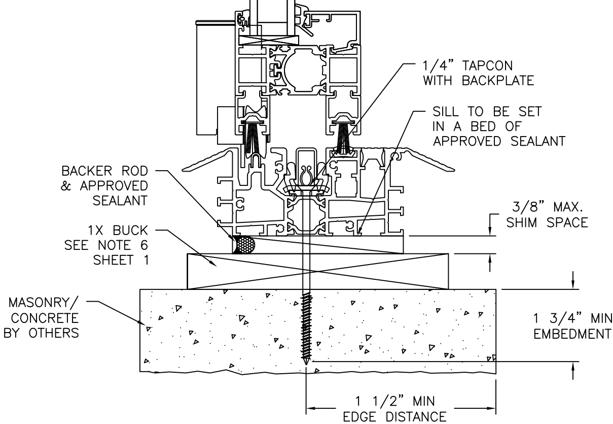
VERTICAL CROSS SECTION MASONRY/CONCRETE W/1X BUCK INSTALLATION SADDLE SILL SHOWN, OTHER SILLS SIMILAR
