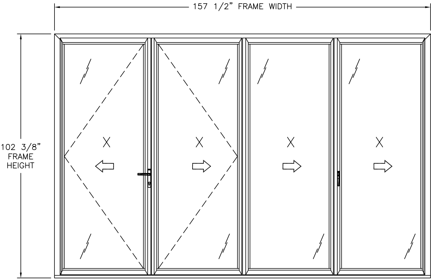
SERIES NW REINFORCED 647 FOLDING PANEL SYSTEM OUTSWING INTERIOR VIEW UNLIMITED NUMBER OF PANELS IN UNLIMITED CONFIGURATIONS ARE APPROVED AS LONG AS INDIVIDUAL PANEL AREA DOES NOT EXCEED 27.62 FT 2
