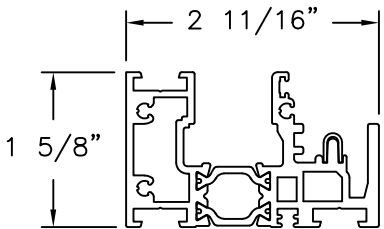
PERFORMANCE SILL ALUMINUM 6063-T5
