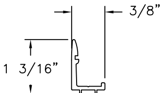
BAR PROFILE (5-300-08) ALUMINUM 6063-T5
