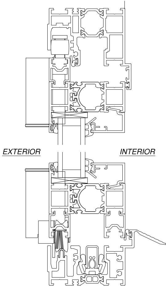
VERTICAL CROSS SECTION WITH HYBRID SILL
