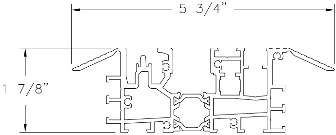
LOW PROFILE SADDLE SILL (5-310-11) ALUMINUM 6063-T5
