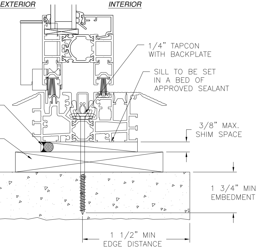
VERTICAL CROSS SECTION MASONRY/CONCRETE W/1X BUCK INSTALLATION HYBRID SILL SHOWN, OTHER SILLS SIMILAR
