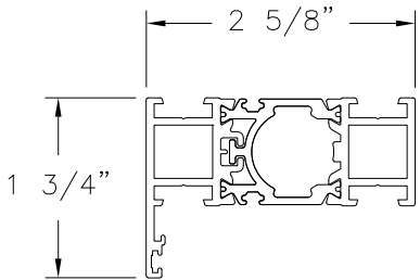
OUTSWING PANEL PROFILE (5-310-02) ALUMINUM 6063-T5
