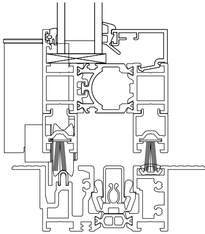
VERTICAL CROSS SECTION WITH EXTENDED HEAD AND FLUSH SILL
