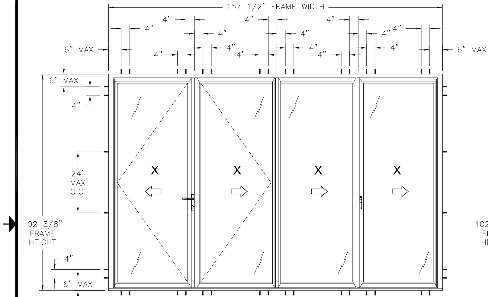
SERIES NW REINFORCED 647 FOLDING PANEL SYSTEM OUTSWING ANCHORING LAYOUT FOR UNITS RATED HIGHER THAN 40PSF
