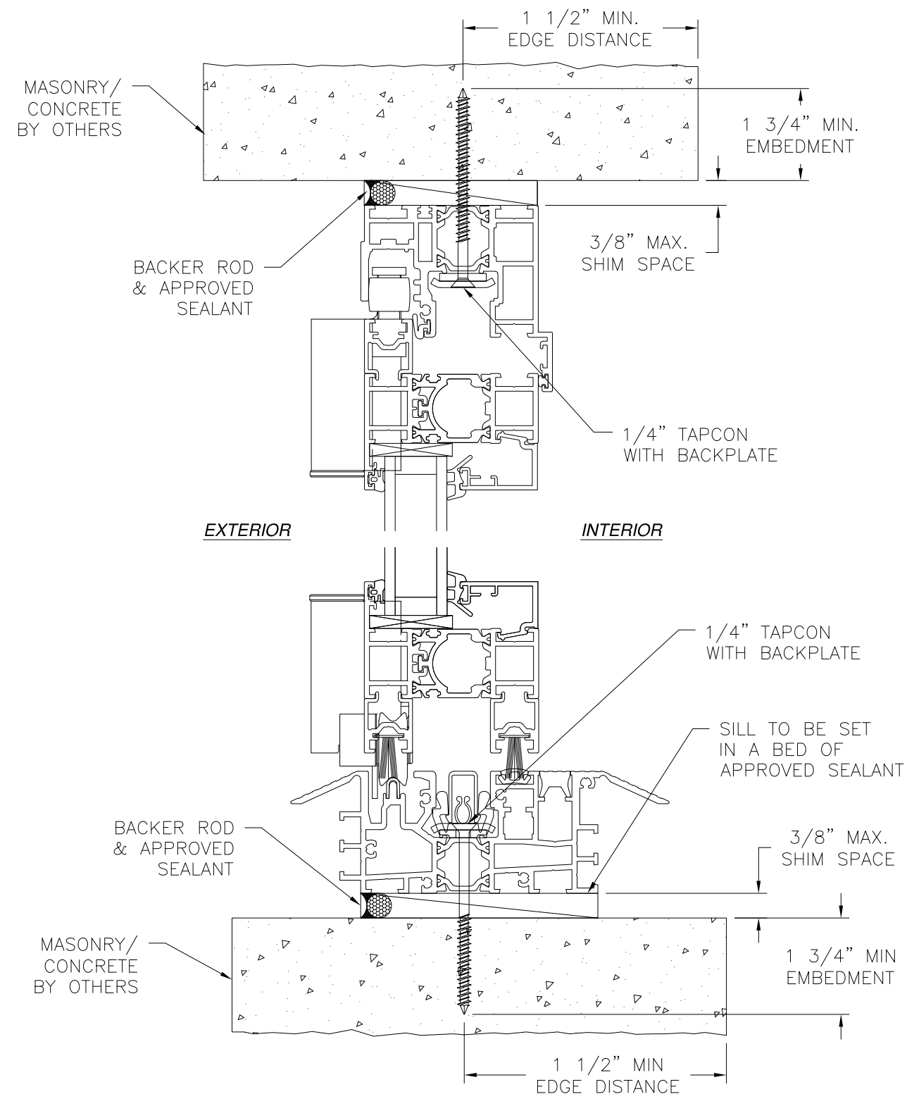
VERTICAL CROSS SECTION MASONRY/CONCRETE INSTALLATION HYBRID SILL SHOWN, OTHER SILLS SIMILAR
