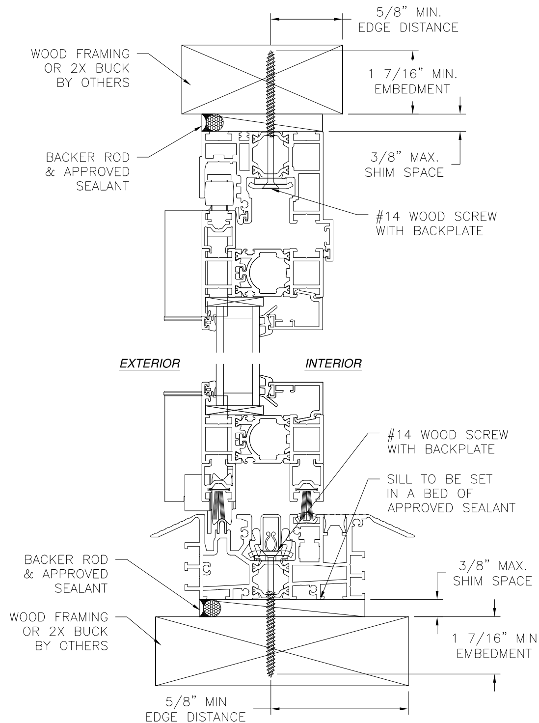
VERTICAL CROSS SECTION WOOD FRAMING OR 2X BUCK INSTALLATION SADDLE SILL SHOWN, OTHER SILLS SIMILAR
