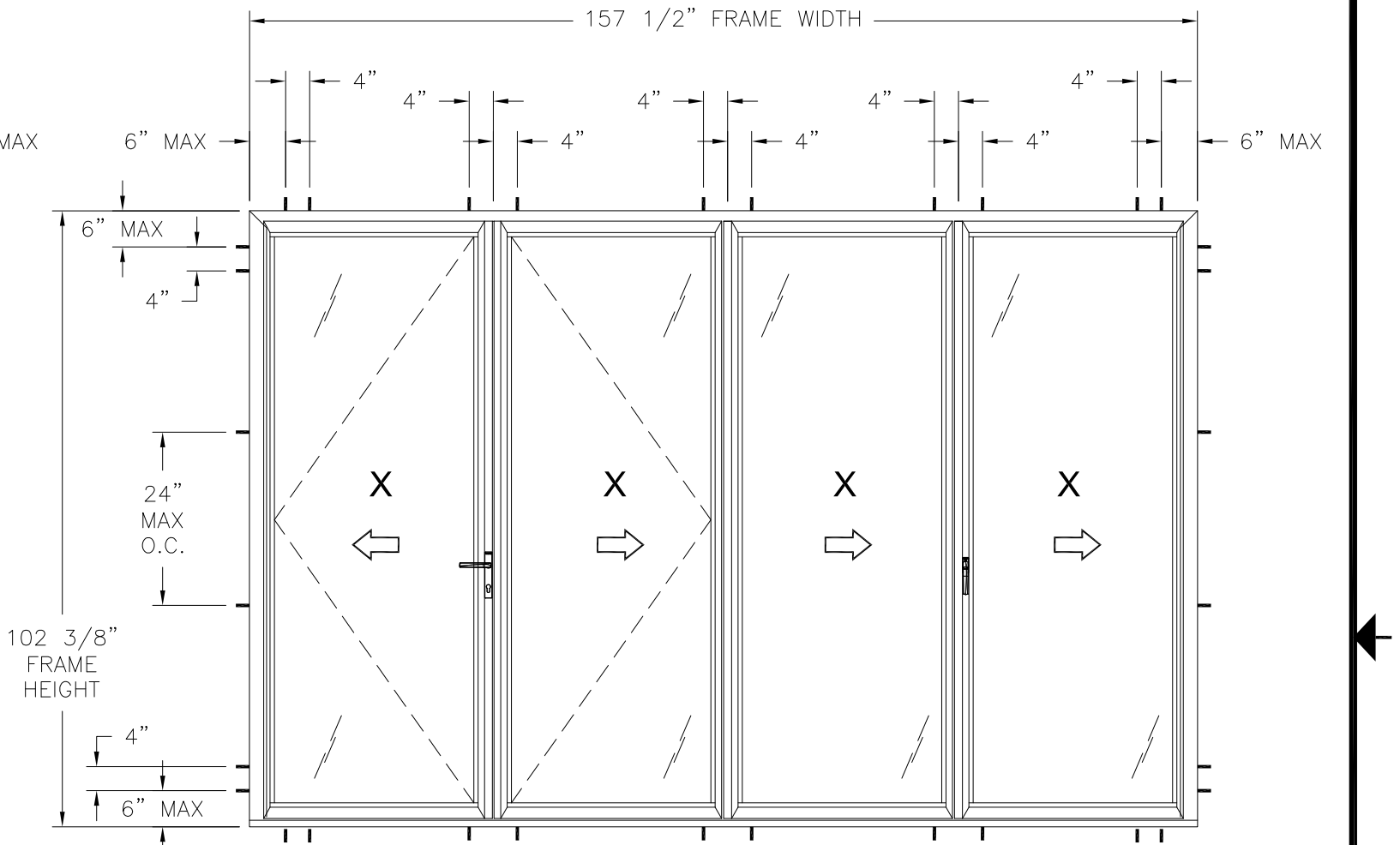
SERIES NW REINFORCED 647 FOLDING PANEL SYSTEM OUTSWING ANCHORING LAYOUT FOR UNITS RATED LOWER THAN 40PSF
