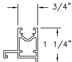
EXTENSION PROFILE (5-420-03) ALUMINUM 6063-T5
