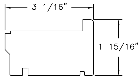
PANEL STILE PROFILE (10-420-6174) 3-4 LAYER SOLID WOOD
