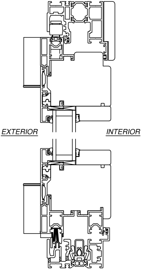
VERTICAL CROSS SECTION WITH PERFORMANCE SILL
