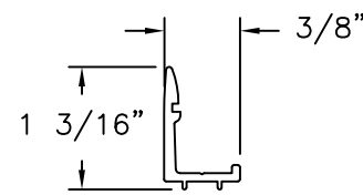
STOP BAR PROFILE (5-300-08) ALUMINUM 6063-T5
