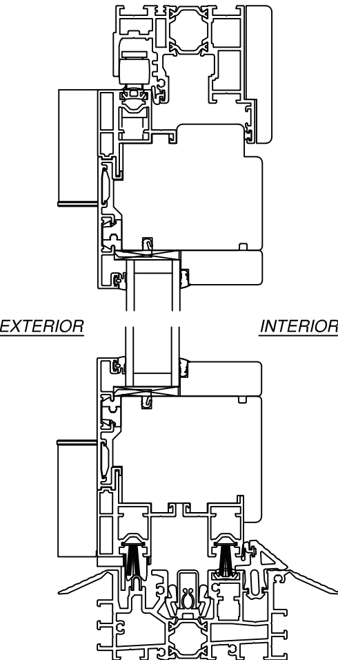
VERTICAL CROSS SECTION WITH UNIVERSILL
