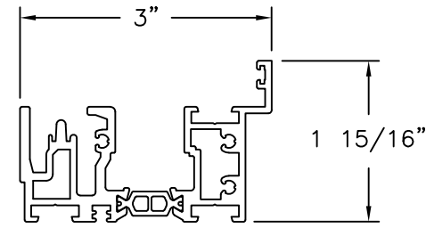
PERFORMANCE SILL ALUMINUM 6063-T5
