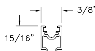
EXTENSION PROFILE (5-300-04) LAMINATED WOOD
