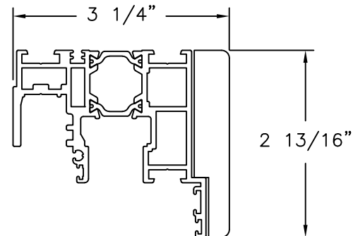
HEAD & JAMB PROFILE (5-310-04) ALUMINUM 6063-T5
