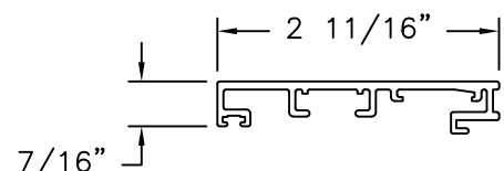
COVER SHELL PROFILE (5-420-01) ALUMINUM 6063-T5
