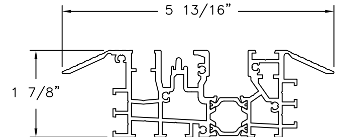
LOW PROFILE SADDLE SILL (5-310-38) ALUMINUM 6063-T5
