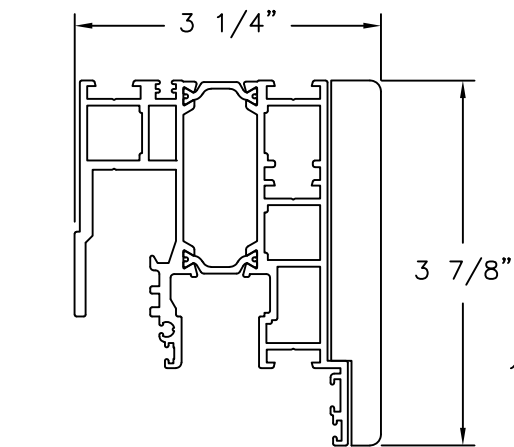
EXTENDED HEAD PROFILE ALUMINUM 6063-T5
