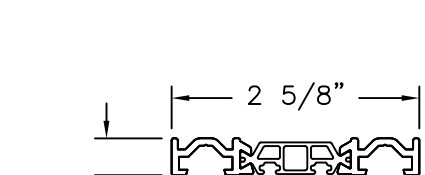
CONNECTING PROFILE (5-400-01) ALUMINUM 6063-T5
