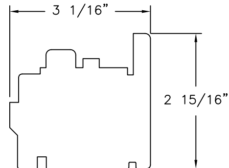
PANEL TOP RAIL PROFILE (10-420-6171) 3-4 LAYER SOLID WOOD
