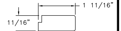
GLAZING BEAD (10-420-01) SOLID WOOD
