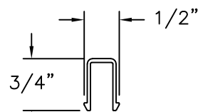
SILL INSERT PROFILE (5-310-26) ALUMINUM 6063-T5
