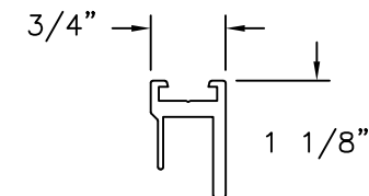
ADJUSTABLE JAMB PROFILE (5-300-01) ALUMINUM 6063-T5
