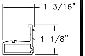
STOP BAR PROFILE (5-450-06) ALUMINUM 6063-T5
