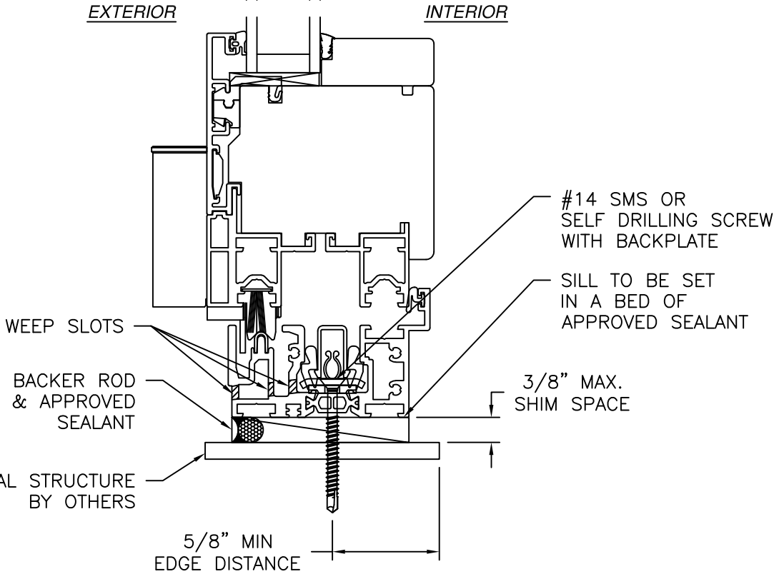
VERTICAL CROSS SECTION METAL STRUCTURE INSTALLATION PERFORMANCE SILL SHOWN, OTHER SILLS SIMILAR
