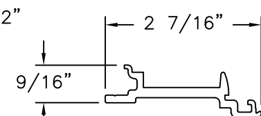
CONNECTION STRIP PROFILE (5-310-27) ALUMINUM 6063-T5
