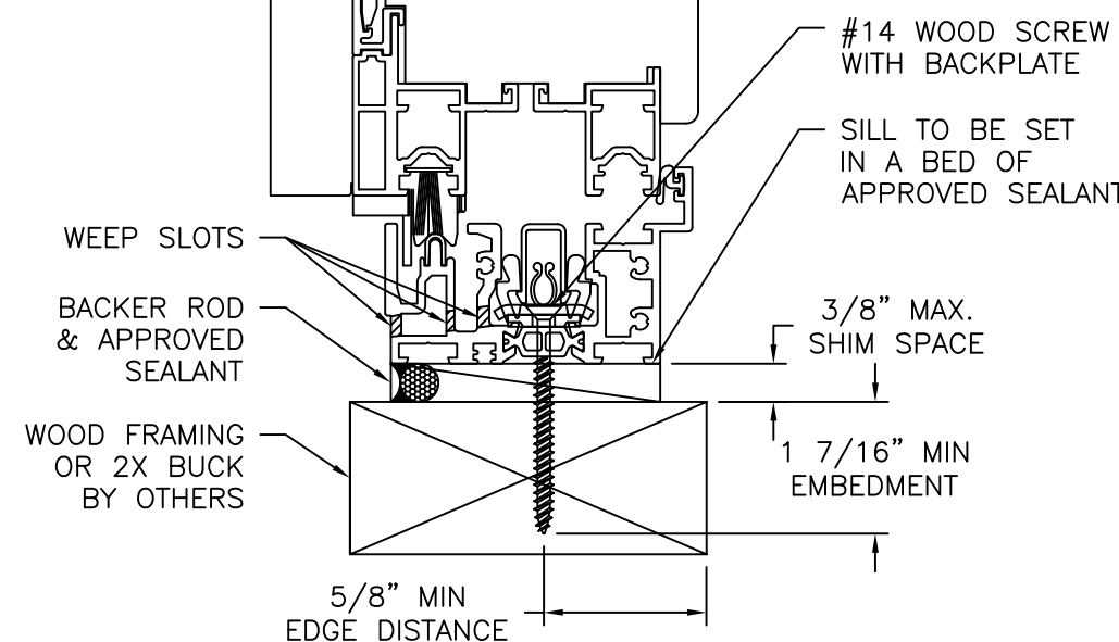
VERTICAL CROSS SECTION WOOD FRAMING OR 2X BUCK INSTALLATION PERFORMANCE SILL SHOWN, OTHER SILLS SIMILAR
