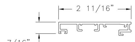
COVER SHELL PROFILE (5-420-01) ALUMINUM 6063-T5
