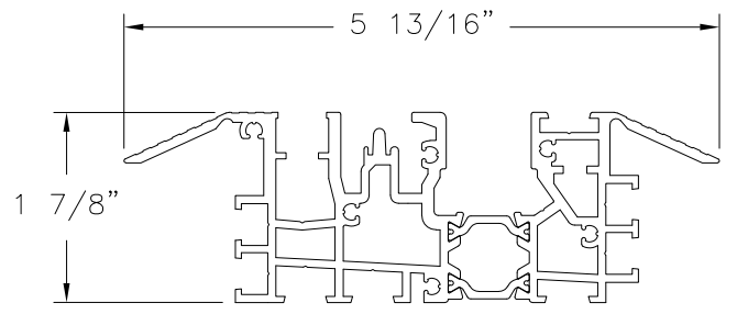
LOW PROFILE SADDLE SILL (5-310-38) ALUMINUM 6063-T5
