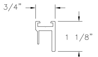
ADJUSTABLE JAMB PROFILE (5-300-01) ALUMINUM 6063-T5
