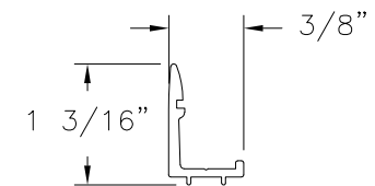
STOP BAR PROFILE (5-300-08) ALUMINUM 6063-T5
