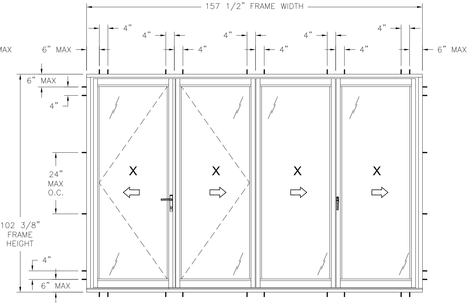
SERIES NW CLAD 740 FOLDING PANEL SYSTEM OUTSWING ANCHORING LAYOUT FOR UNITS RATED LOWER THAN 40PSF
