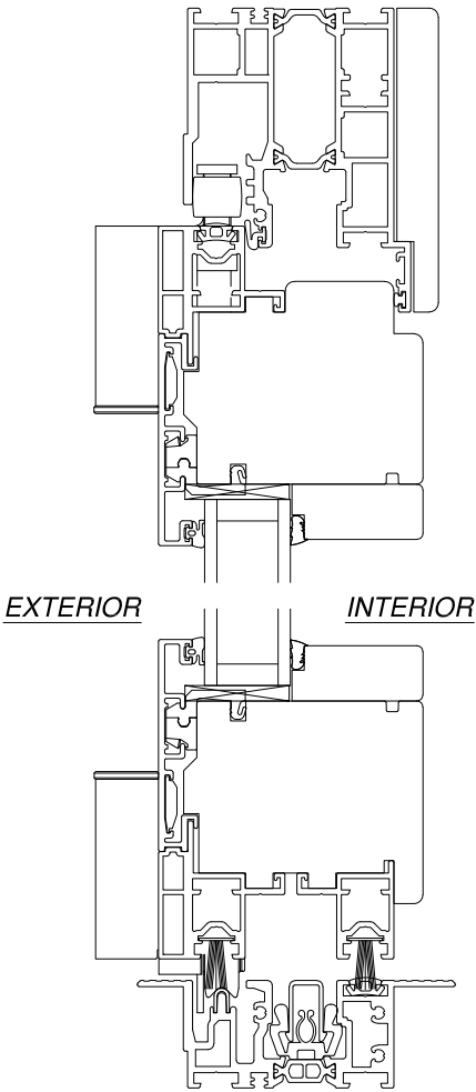
VERTICAL CROSS SECTION WITH EXTENDED HEAD AND FLUSH SILL
