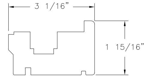
PANEL STILE PROFILE AT LOCKING SIDE (10-420-6175) 3-4 LAYER SOLID WOOD
