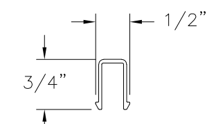
SILL INSERT PROFILE (5-310-26) ALUMINUM 6063-T5
