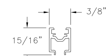
EXTENSION PROFILE (5-300-04) LAMINATED WOOD
