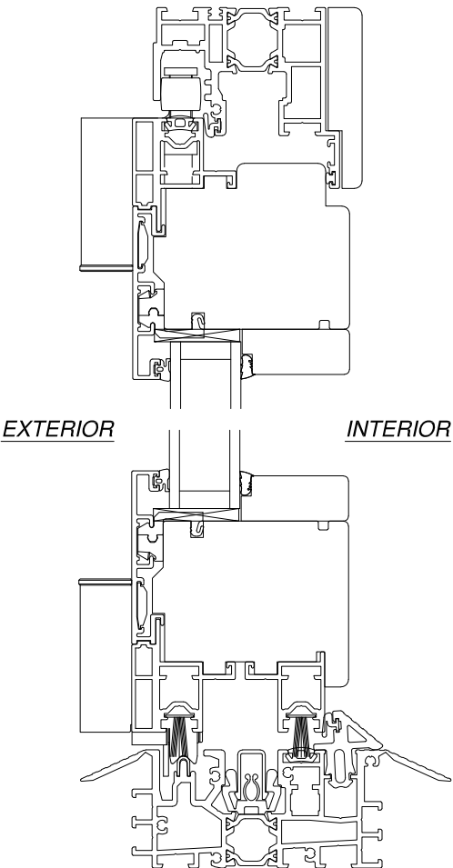
VERTICAL CROSS SECTION WITH UNIVERSILL
