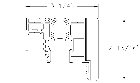
HEAD & JAMB PROFILE (5-310-04) ALUMINUM 6063-T5
