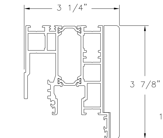
EXTENDED HEAD PROFILE ALUMINUM 6063-T5
