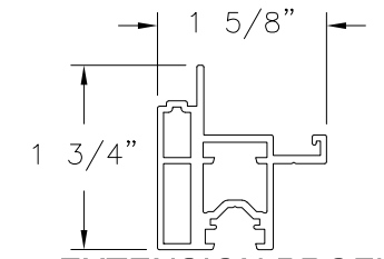
EXTENSION PROFILE (5-420-04) ALUMINUM 6063-T5
