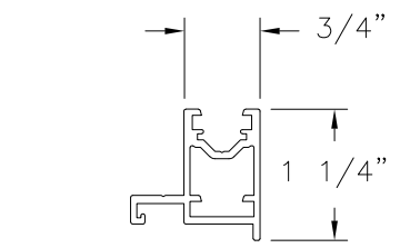
EXTENSION PROFILE (5-420-03) ALUMINUM 6063-T5
