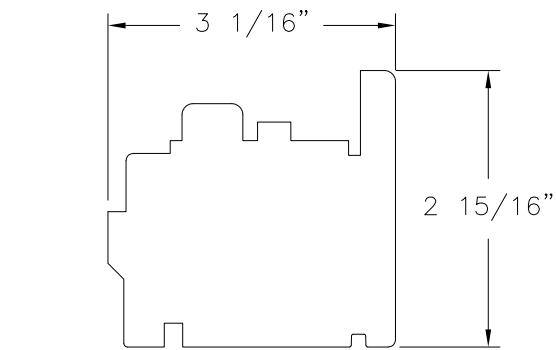
PANEL TOP RAIL PROFILE (10-420-6171) 3-4 LAYER SOLID WOOD
