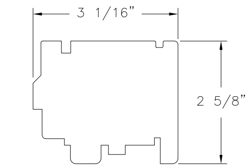
PANEL BOTTOM RAIL PROFILE (10-420-6172) 3-4 LAYER SOLID WOOD
