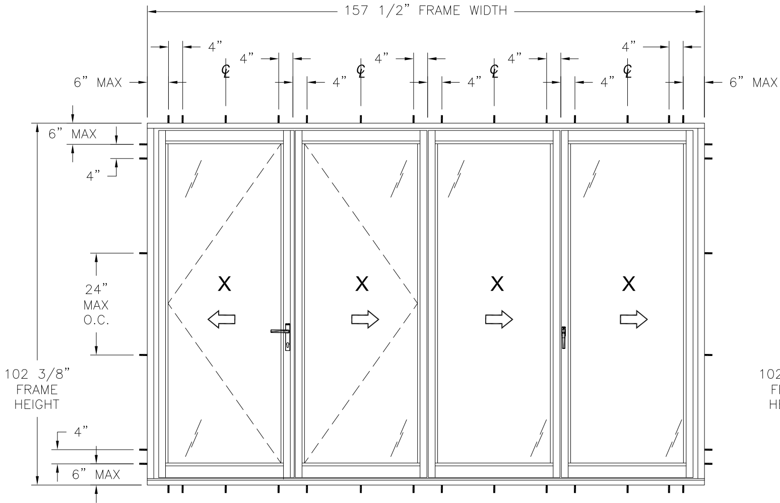
SERIES NW CLAD 740 FOLDING PANEL SYSTEM OUTSWING ANCHORING LAYOUT FOR UNITS RATED HIGHER THAN 40PSF
