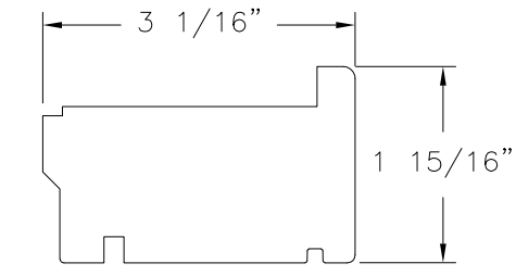
PANEL STILE PROFILE (10-420-6174) 3-4 LAYER SOLID WOOD
