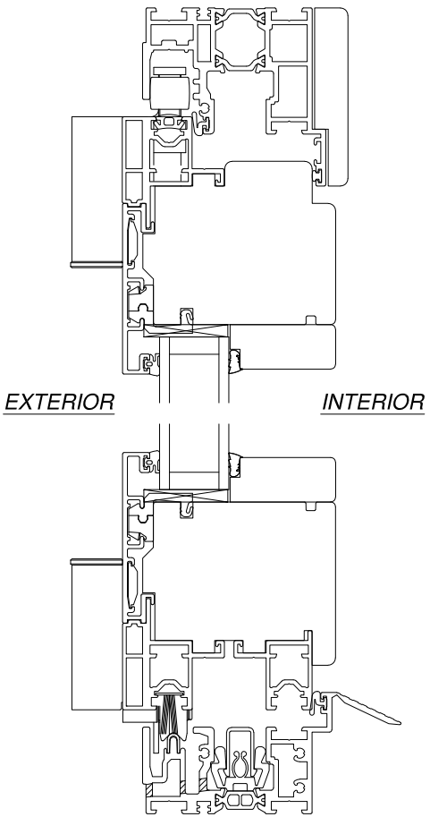
VERTICAL CROSS SECTION WITH HYBRID SILL
