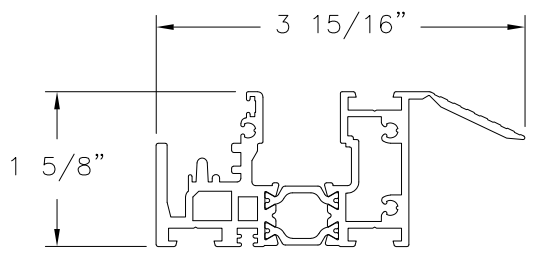
HYBRID SILL ALUMINUM 6063-T5
