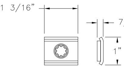
BACK PLATE (15-310-40) STEEL
