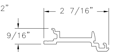
CONNECTION STRIP PROFILE (5-310-27) ALUMINUM 6063-T5
