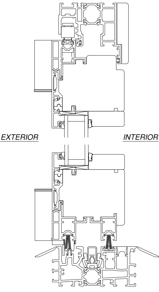
VERTICAL CROSS SECTION WITH SADDLE SILL
