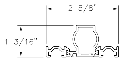
CONNECTING PROFILE (5-400-02) ALUMINUM 6063-T5
