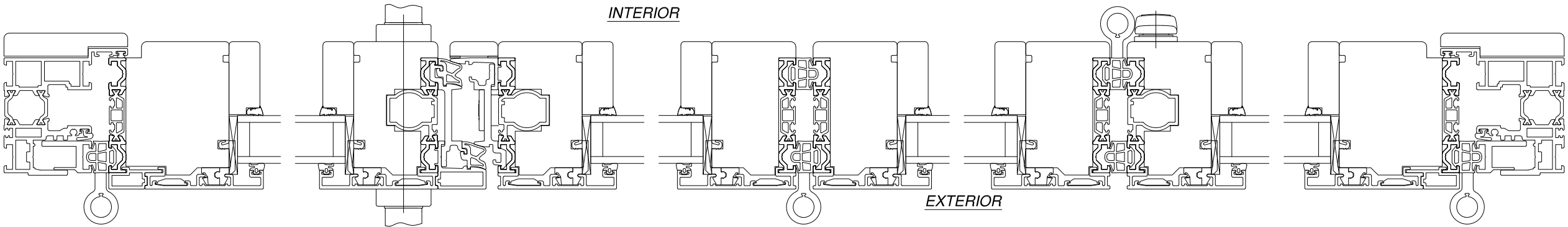
HORIZONTAL CROSS SECTION
