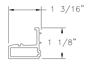
STOP BAR PROFILE (5-450-06) ALUMINUM 6063-T5
