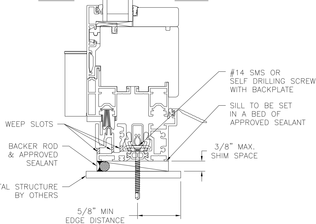
VERTICAL CROSS SECTION METAL STRUCTURE INSTALLATION HYBRID SILL SHOWN, OTHER SILLS SIMILAR
