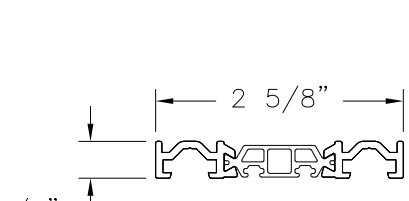
CONNECTING PROFILE (5-400-01) ALUMINUM 6063-T5
