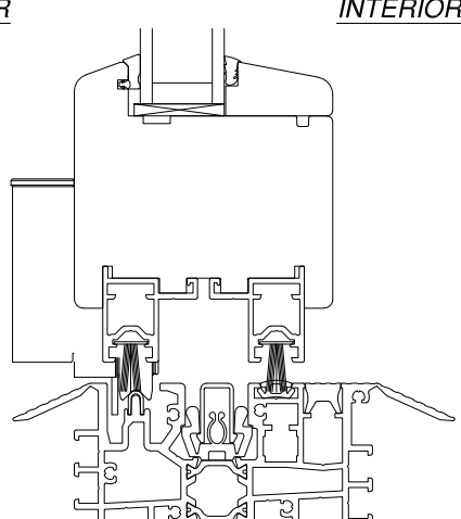
VERTICAL CROSS SECTION WITH SADDLE SILL
