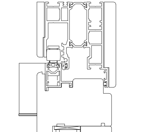
EXTERIOR INTERIOR
