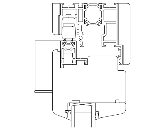
EXTERIOR INTERIOR
