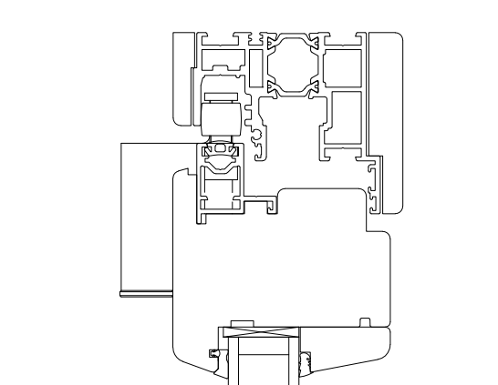
EXTERIOR INTERIOR
