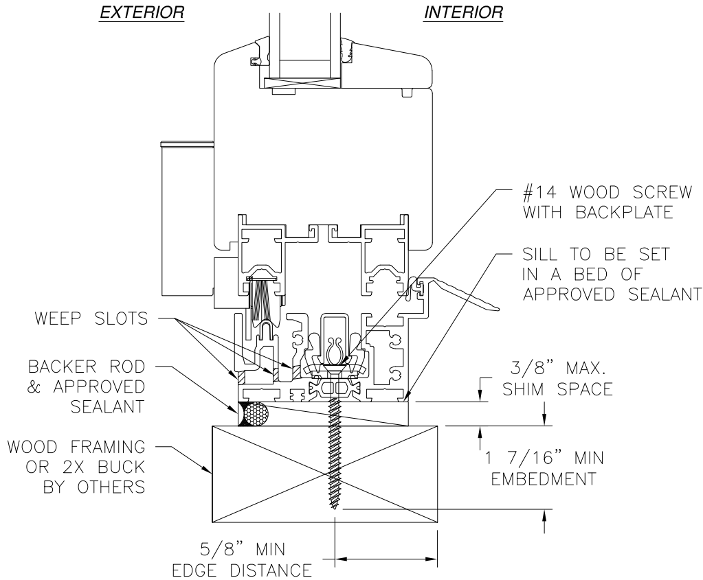
VERTICAL CROSS SECTION WOOD FRAMING OR 2X BUCK INSTALLATION HYBRID SILL SHOWN, OTHER SILLS SIMILAR
