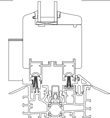
VERTICAL CROSS SECTION WITH UNIVERSILL
