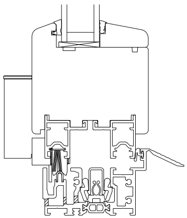
VERTICAL CROSS SECTION WITH HYBRID SILL
