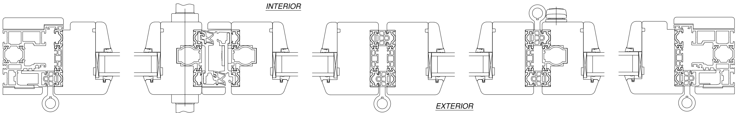
HORIZONTAL CROSS SECTION
