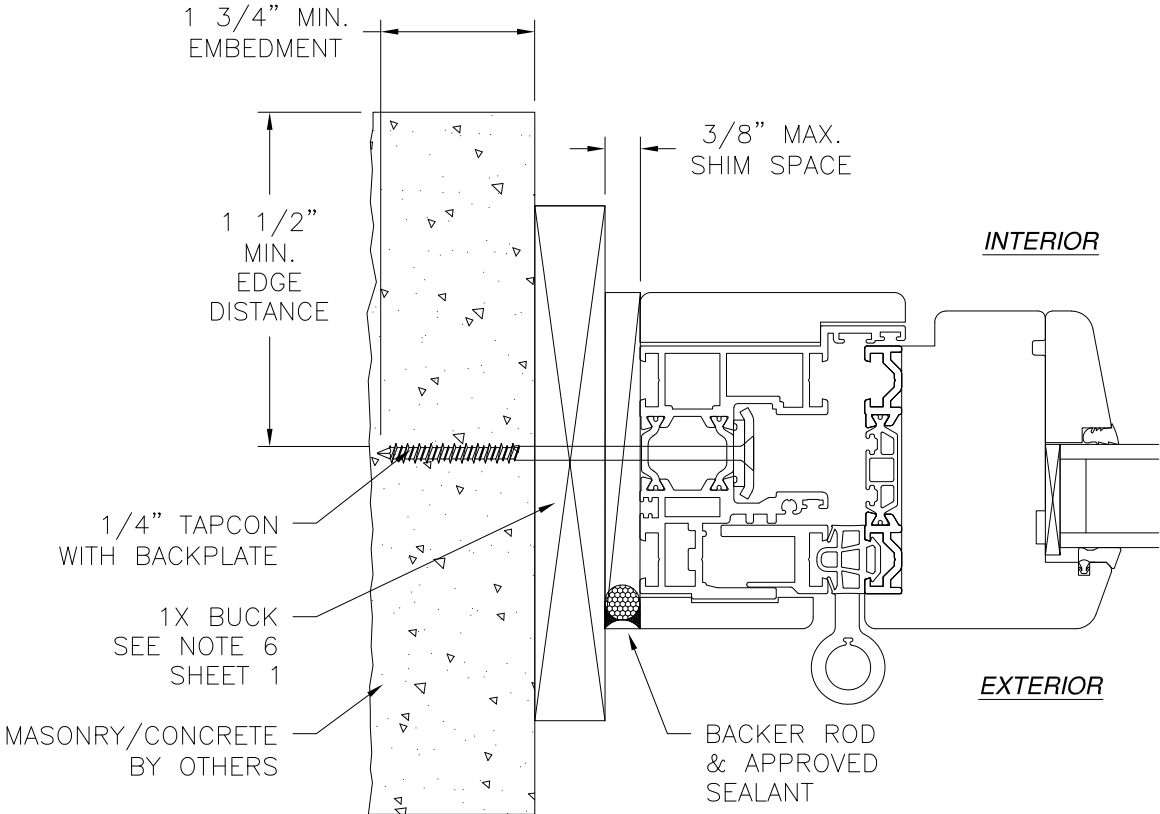
JAMB INSTALLATION DETAIL MASONRY/CONCRETE W/1X BUCK INSTALLATION
