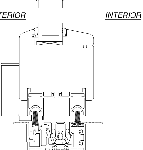
VERTICAL CROSS SECTION WITH EXTENDED HEAD AND FLUSH SILL
