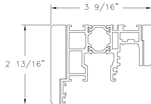
HEAD & JAMB PROFILE (5-310-04) ALUMINUM 6063-T5
