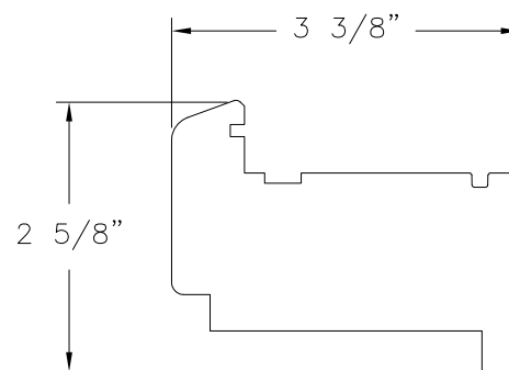
PANEL STILE PROFILE AT JAMB (10-410-6184) 3-4 LAYER SOLID WOOD
