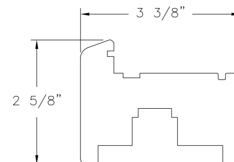
PANEL STILE PROFILE AT LOCKING SIDE (10-410-6185) 3-4 LAYER SOLID WOOD
