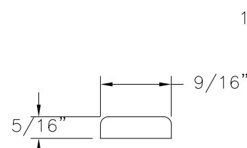
COVER PROFILE (10-400-21) LAMINATED WOOD
