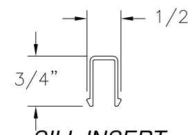
SILL INSERT PROFILE (5-310-26) ALUMINUM 6063-T5
