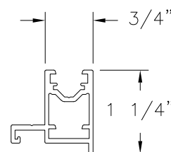
EXTENSION PROFILE (5-420-03) ALUMINUM 6063-T5
