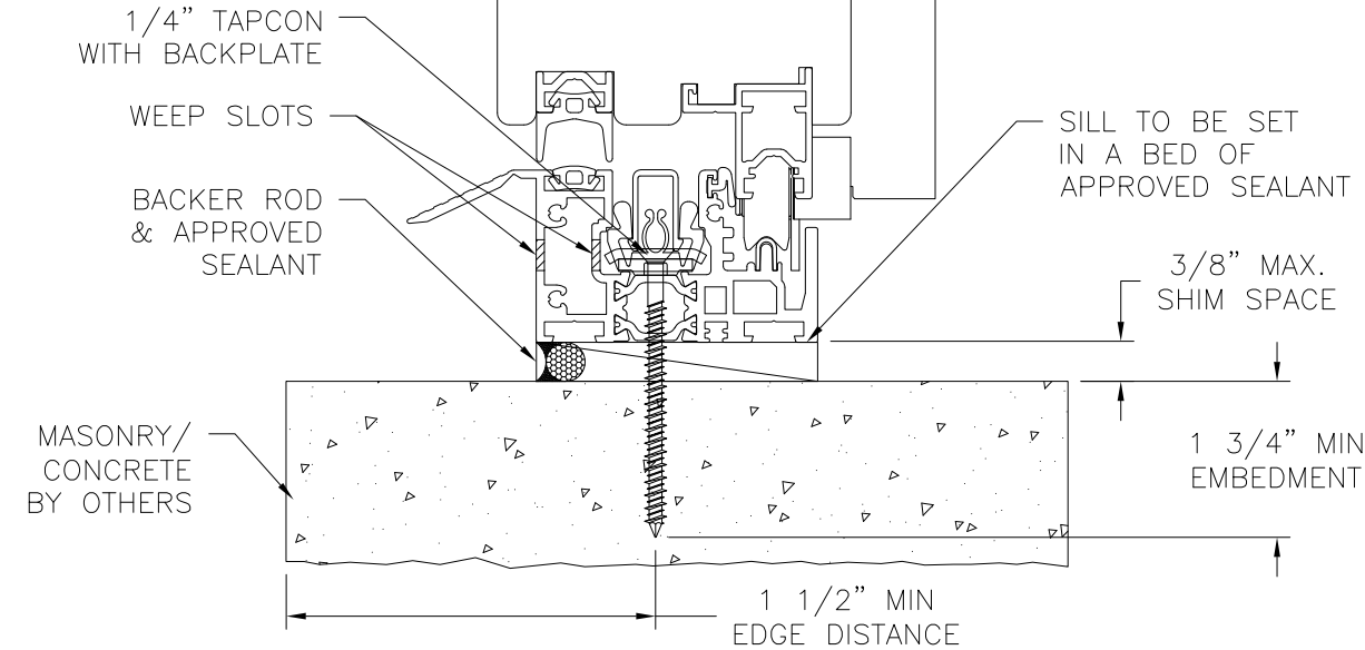
VERTICAL CROSS SECTION MASONRY/CONCRETE INSTALLATION HYBRID SILL SHOWN, OTHER SILLS SIMILAR
