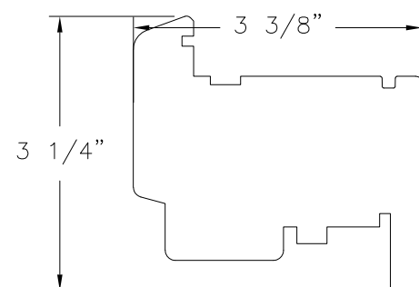
PANEL TOP RAIL PROFILE (10-410-6181) 3-4 LAYER SOLID WOOD
