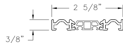
CONNECTING PROFILE (5-400-01) ALUMINUM 6063-T5
