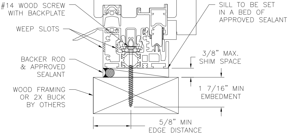
VERTICAL CROSS SECTION WOOD FRAMING OR 2X BUCK INSTALLATION HYBRID SILL SHOWN, OTHER SILLS SIMILAR
