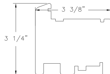
PANEL BOTTOM RAIL PROFILE (10-420-6173) 3-4 LAYER SOLID WOOD
