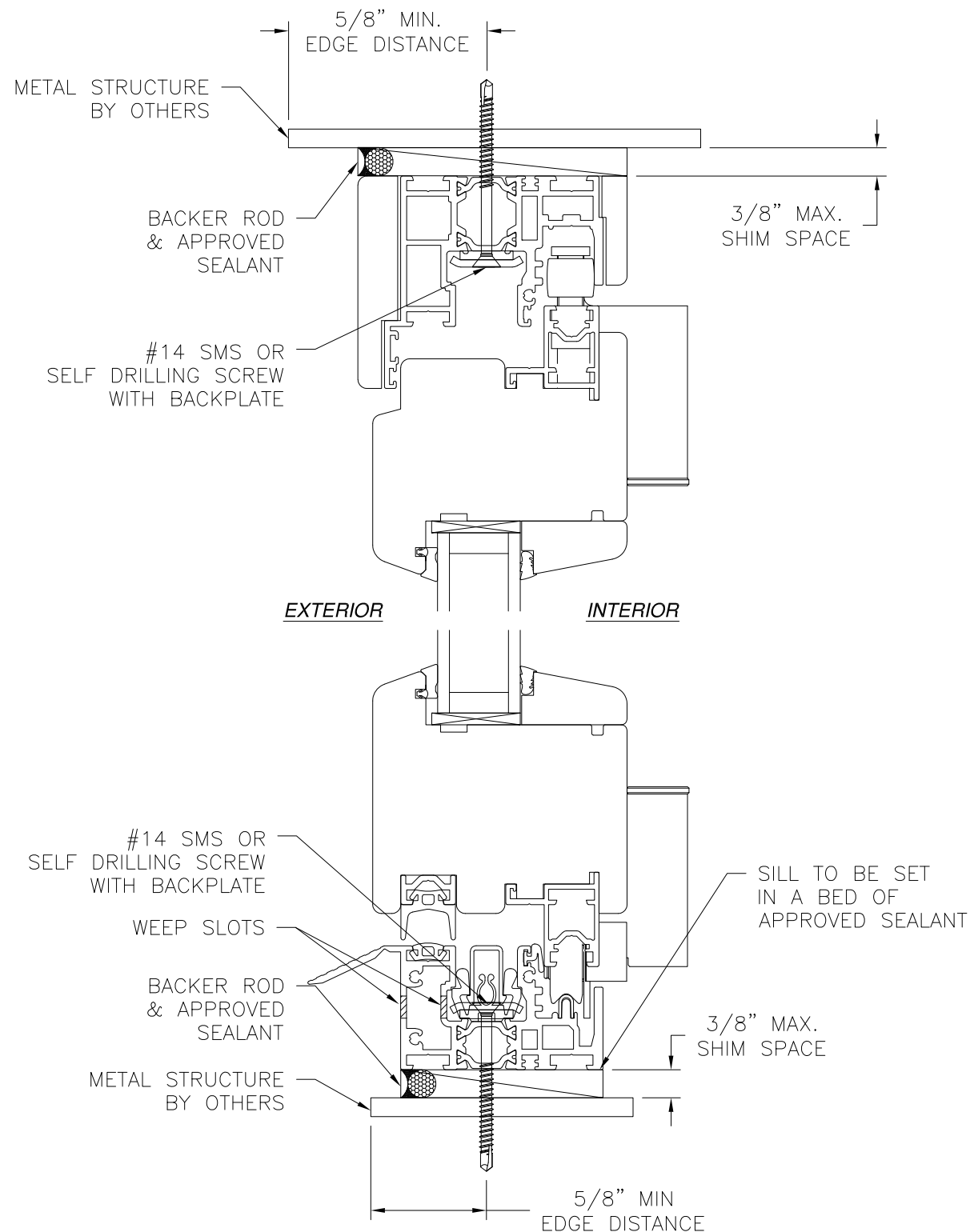
VERTICAL CROSS SECTION METAL STRUCTURE INSTALLATION HYBRID SILL SHOWN, OTHER SILLS SIMILAR
