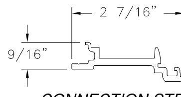
CONNECTION STRIP PROFILE (5-310-27) POLYAMIDE
