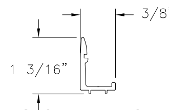
STOP BAR PROFILE (5-300-08) ALUMINUM 6063-T5
