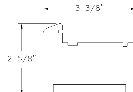
PANEL STILE PROFILE (10-420-6177) 3-4 LAYER SOLID WOOD
