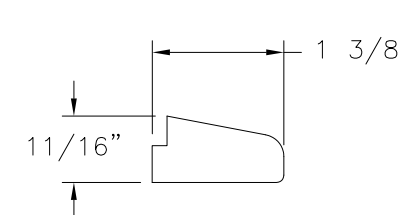
GLAZING BEAD (10-410-01) SOLID WOOD
