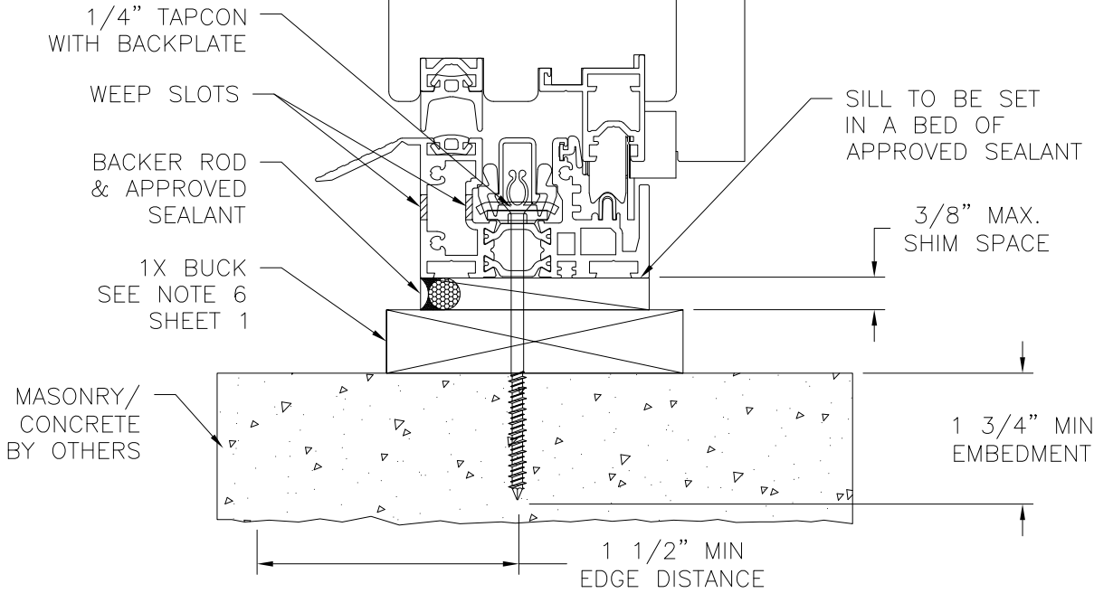
VERTICAL CROSS SECTION MASONRY/CONCRETE W/1X BUCK INSTALLATION HYBRID SILL SHOWN, OTHER SILLS SIMILAR
