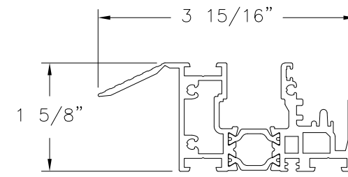
HYBRID SILL ALUMINUM 6063-T5
