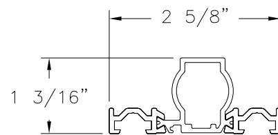
CONNECTING PROFILE (5-400-02) ALUMINUM 6063-T5
