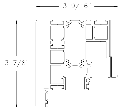
EXTENDED HEAD PROFILE ALUMINUM 6063-T5
