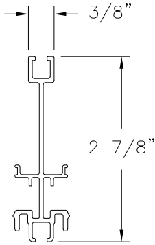
REINFORCEMENT ALUMINUM (T-13468)
