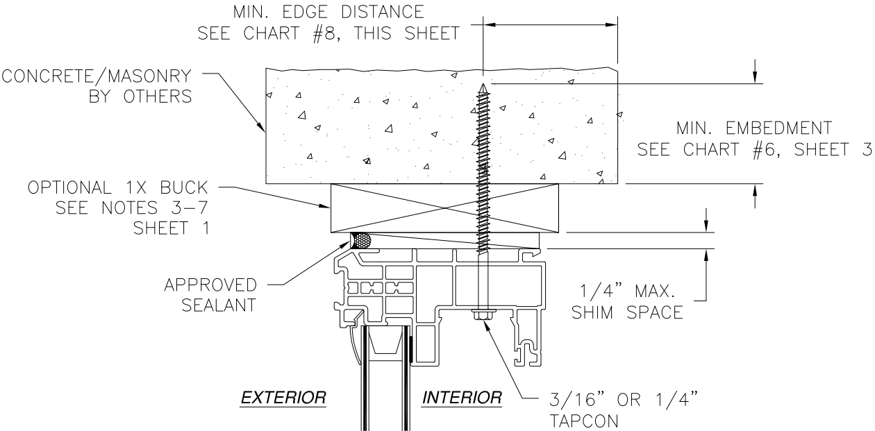
INSTALLATION DETAIL CONCRETE/MASONRY
