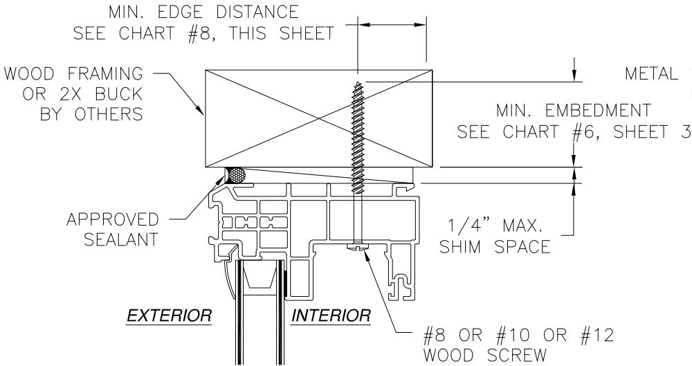
INSTALLATION DETAIL WOOD FRAMING OR 2X BUCK
