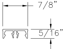
INSIDE COVER CAP PVC (2111)
