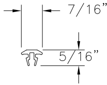
OUTSIDE COVER CAP PVC (2110)
