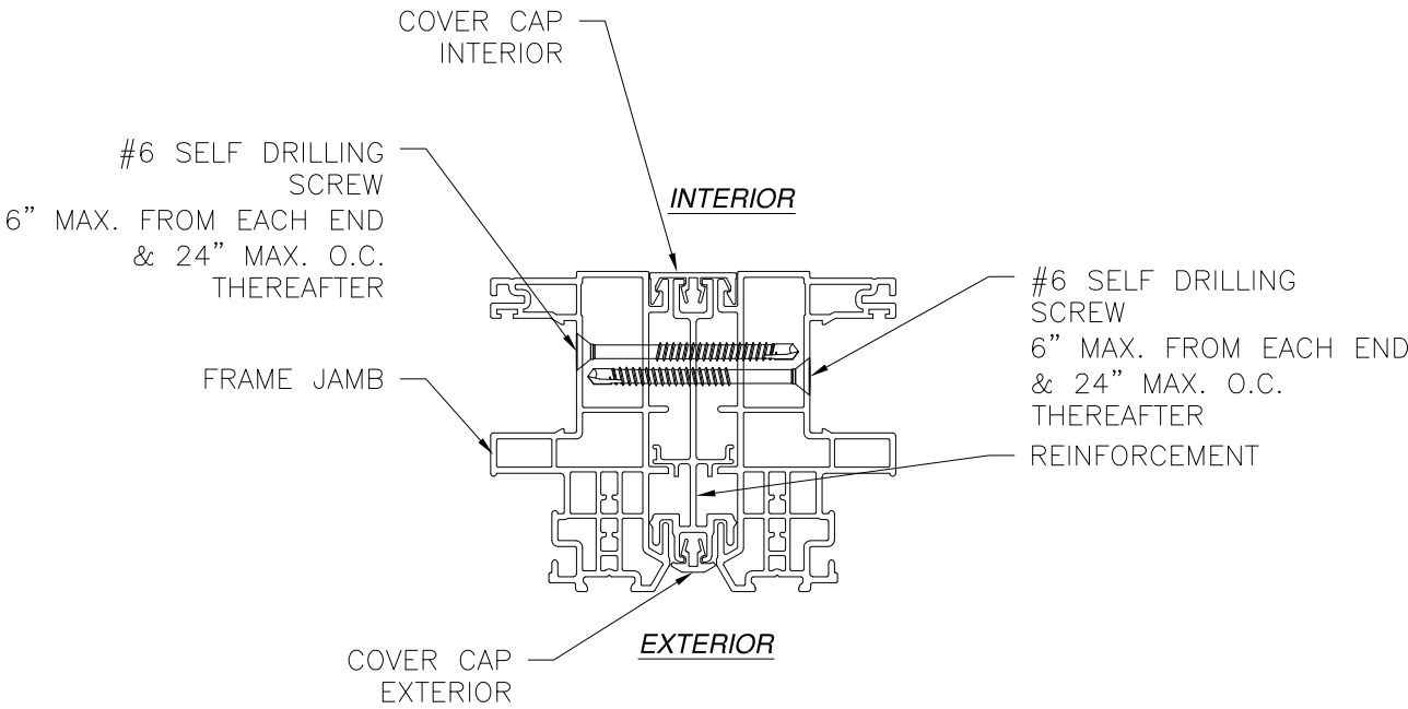
JAMB CONNECTION DETAIL
