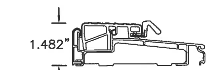
Z-SERIES O/S THRESHOLD
