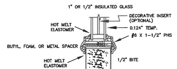
TYPICAL GLAZING DETAIL NON-IMPACT GLASS
