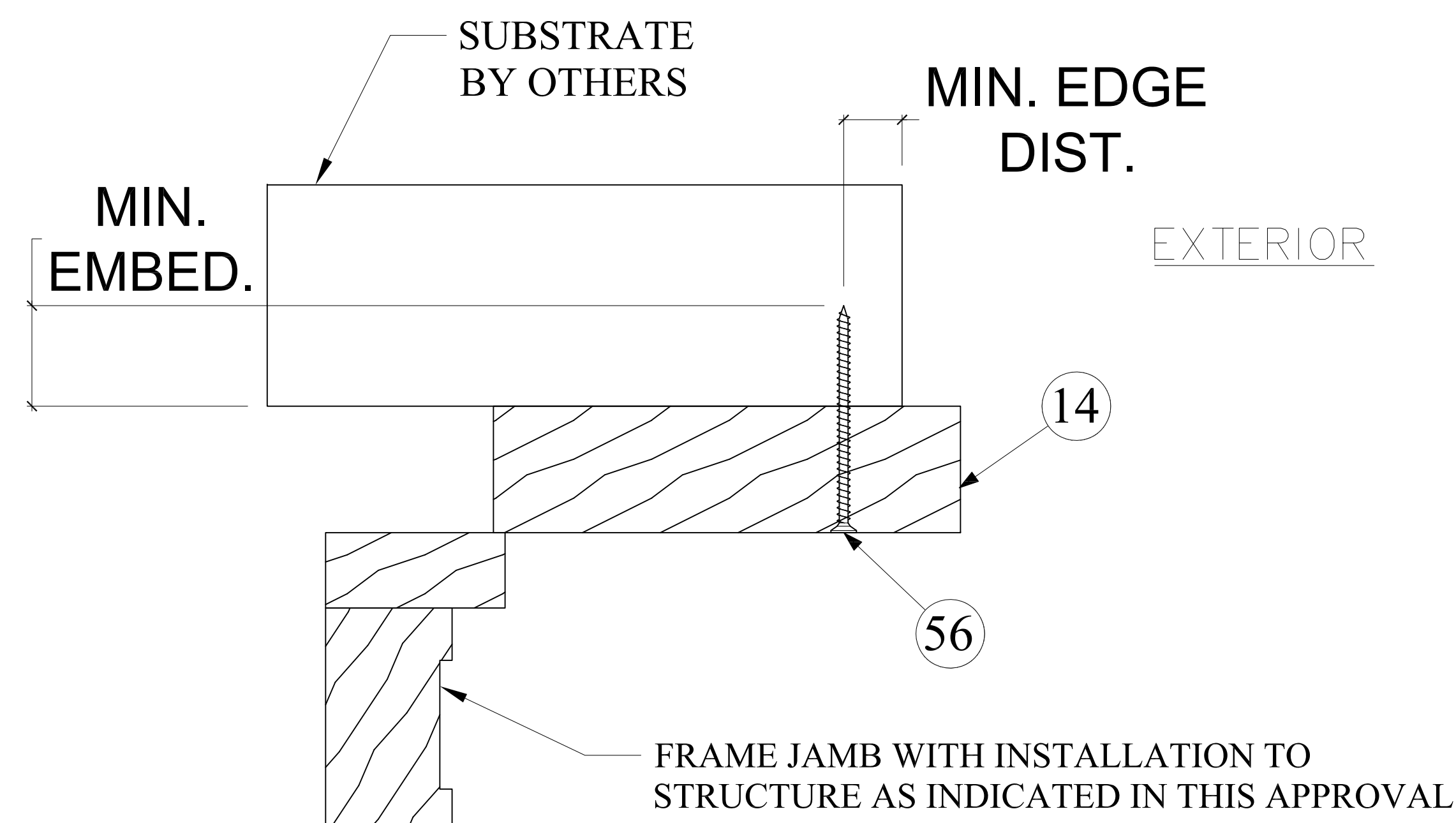
4 POCKET SEALING RAIL SUPPORT INSTALLATION D7
