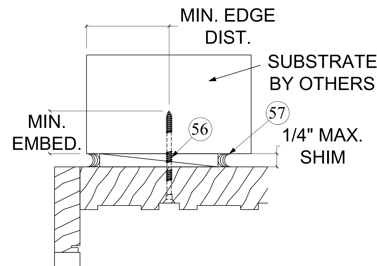
1 HEADER AND JAMB INSTALLATION, THROUGH FRAME D7 APPLIES TO INTERIOR AND/OR EXTERIOR OF FRAMING
