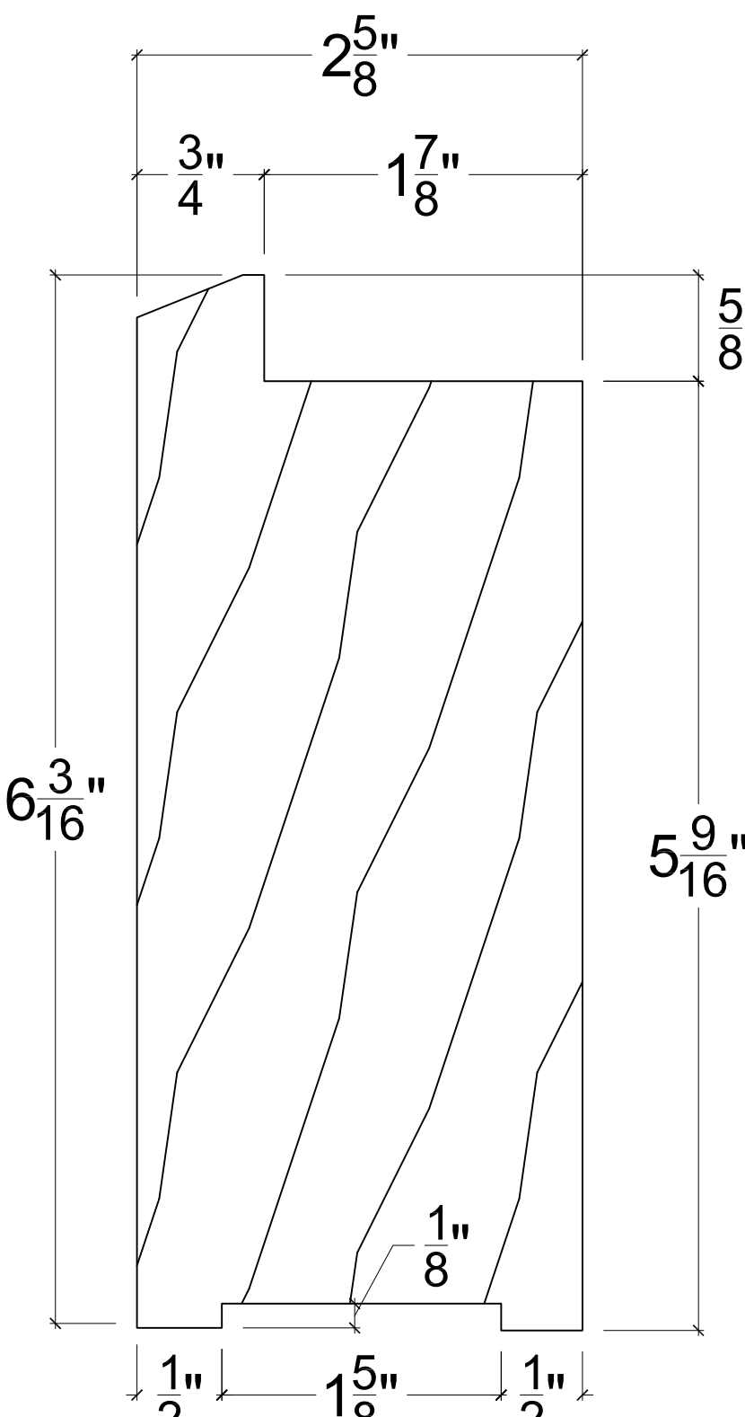
7A BOTTOM RAIL - FIXED D8 1'-0" = 1'-0"
