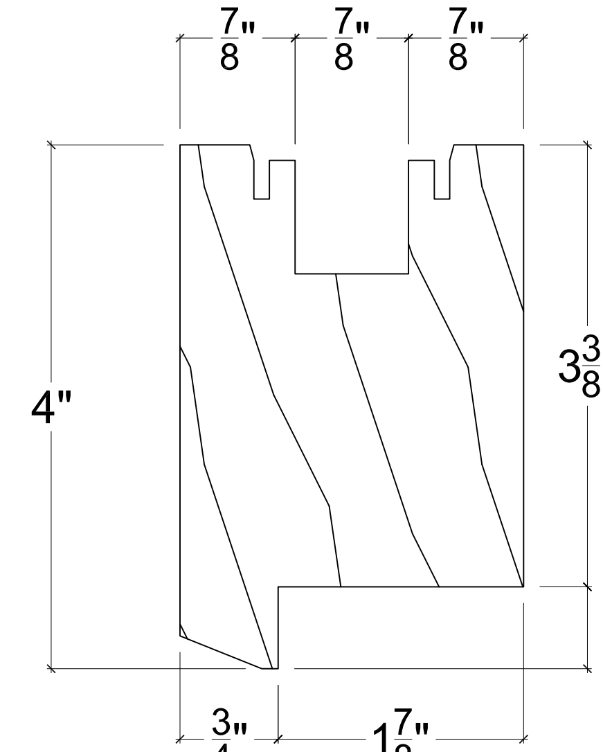
3 TOP RAIL - OPERABLE D8 1'-0" = 1'-0"
