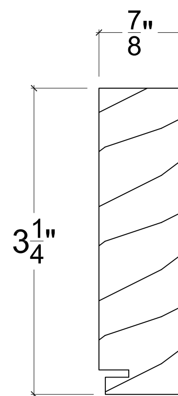
5 HEADER SASH STOP - INTERIOR D8 1'-0" = 1'-0"
