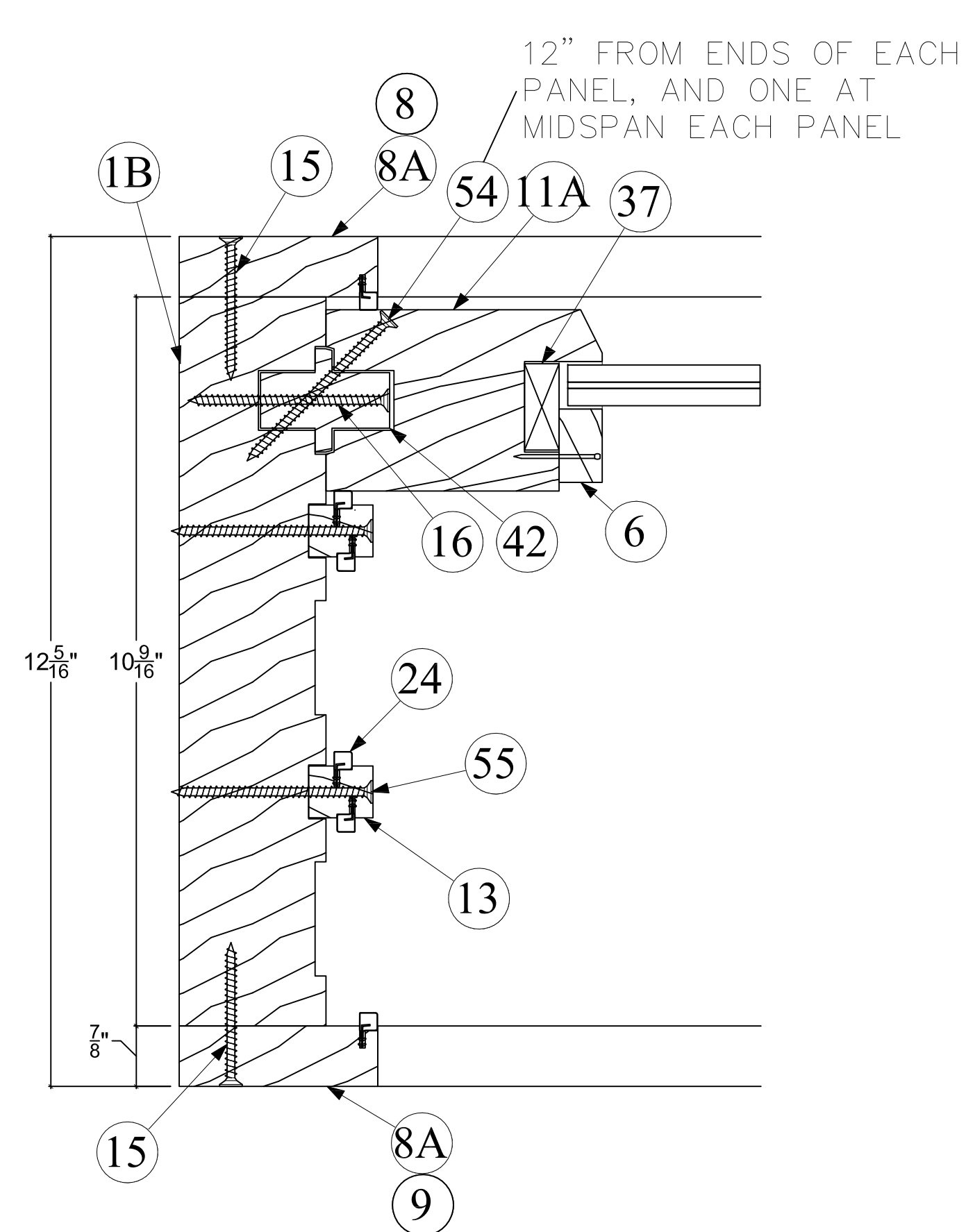
3 D5 FIXED JAMB (3-TRACK SHOWN) (FIXED PANEL OTHER TRACK QTY. SIMILAR, FIXED PANEL MAY BE AT ANY POSITION ON FRAME JAMB)
