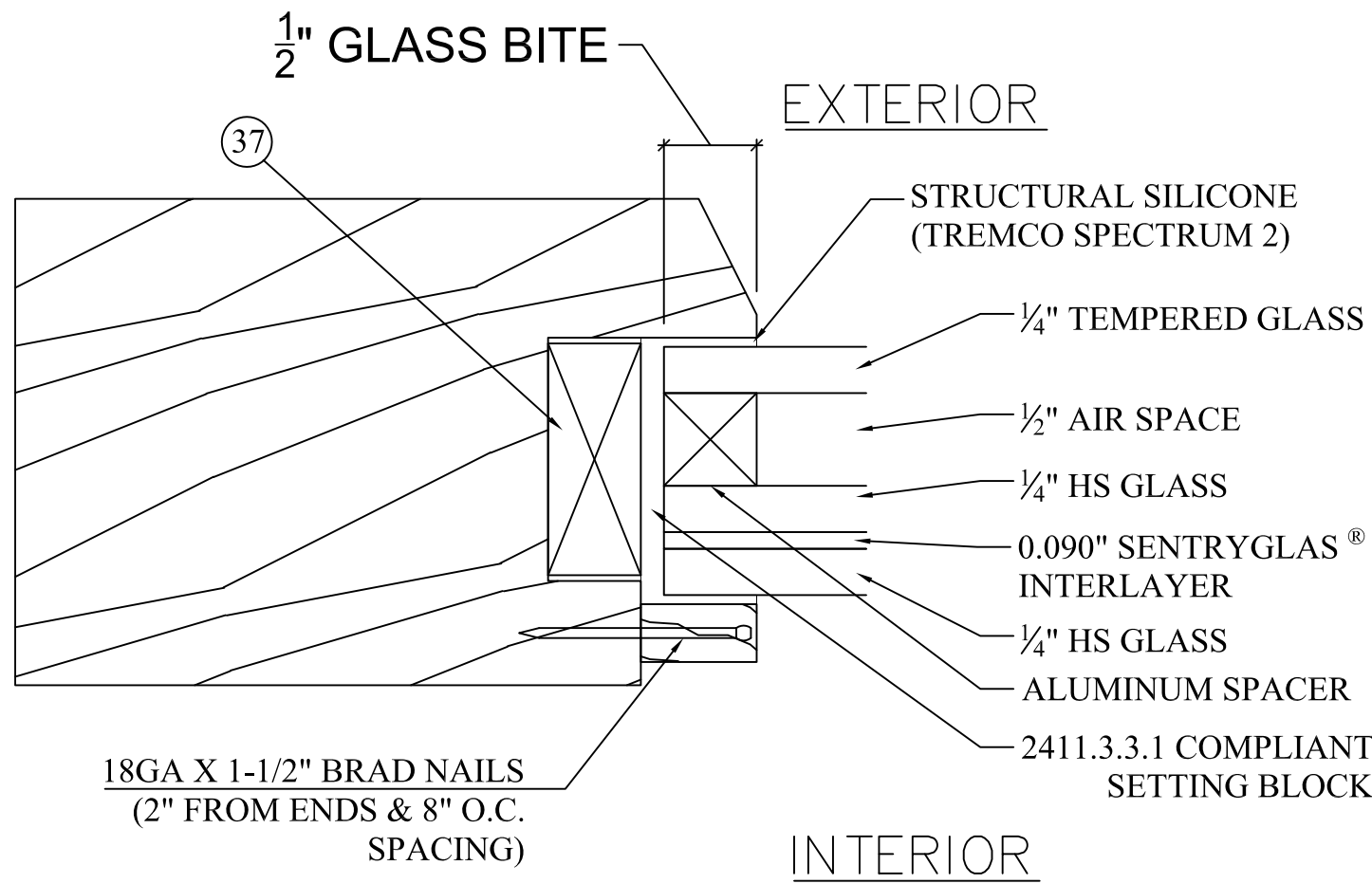
G2 GLAZING DETAILS - 1 3/8" INSULATED GLASS D1 1'-0" = 1'-0"
