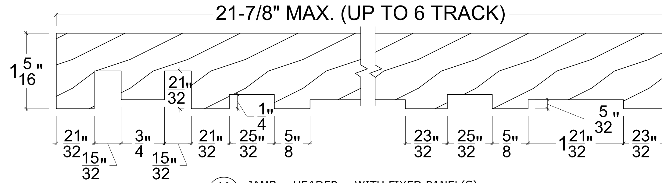
1A JAMB - HEADER - WITH FIXED PANEL(S) D8 1'-0" = 1'-0"
