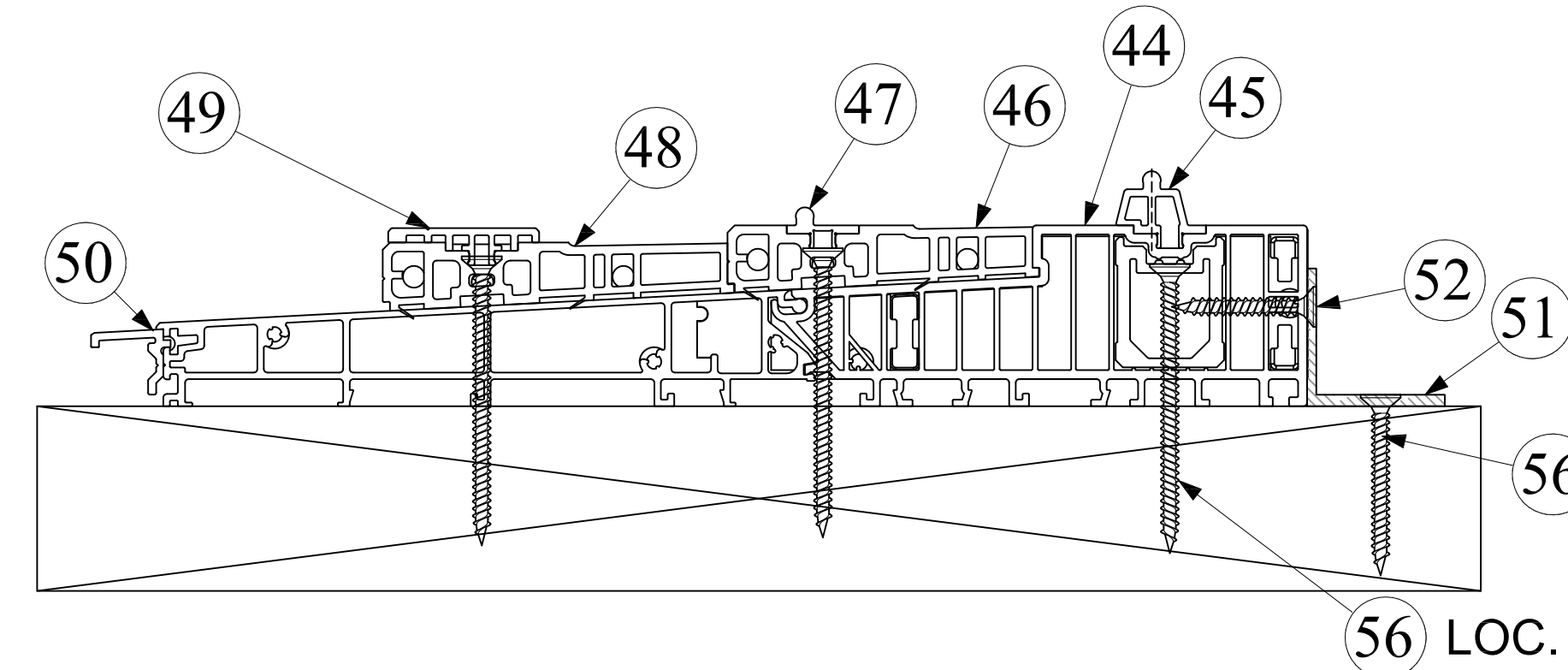
1 SIEGENIA THRESHOLD DETAILS D6 3-TRACK OXX FRAME SHOWN, OTHER SIEGENIA CONFIGURATIONS SIMILAR.
