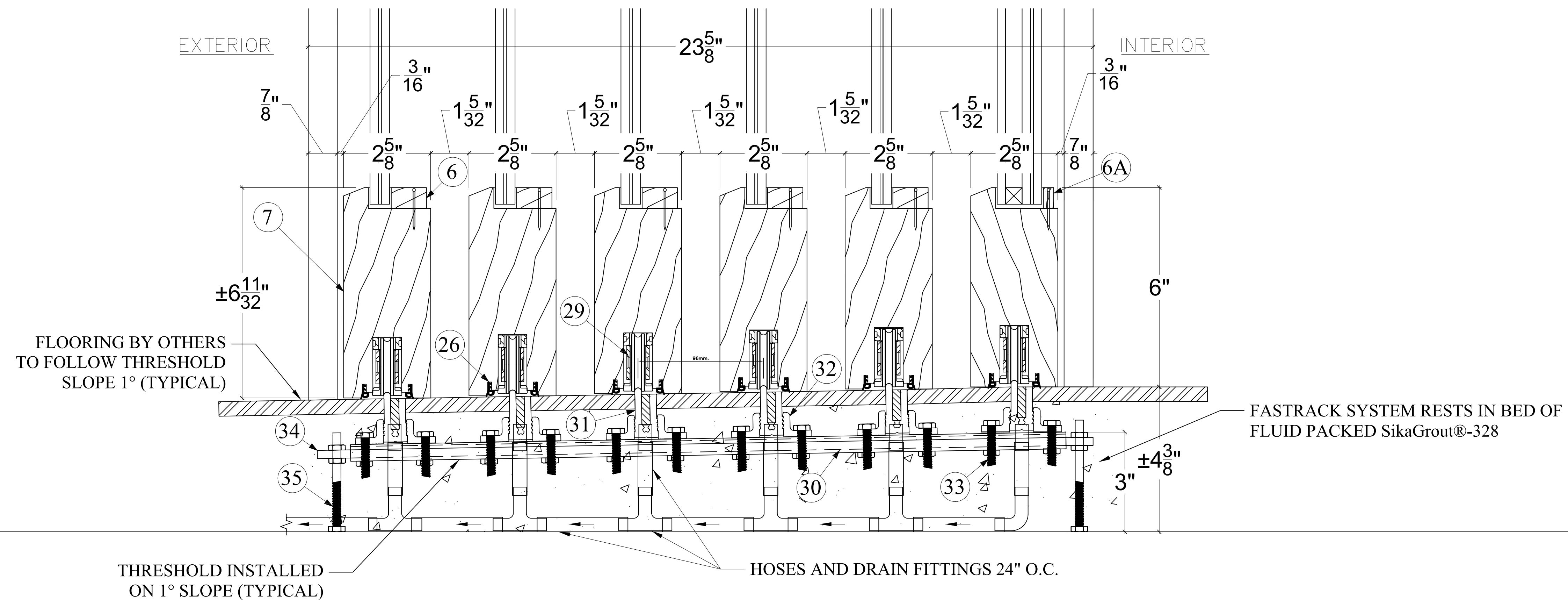
2 FFI FASTRACK THRESHOLD DETAILS D6 6-PANEL POCKET FRAME SHOWN, OTHER FFI CONFIGURATIONS SIMILAR.
