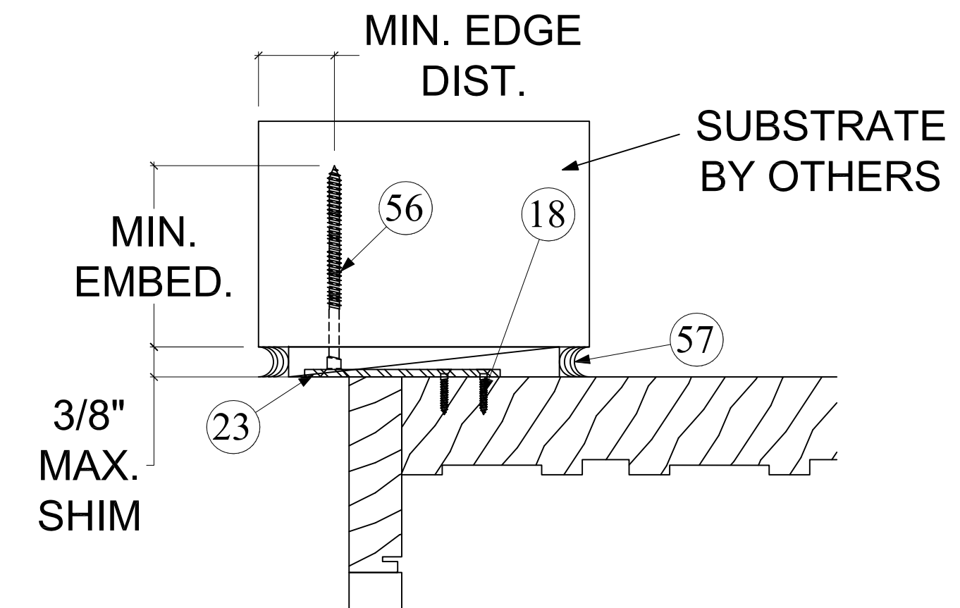
3 HEADER AND JAMB INSTALLATION, FLAT STRAP D7 APPLIES TO INTERIOR AND/OR EXTERIOR OF FRAMING
