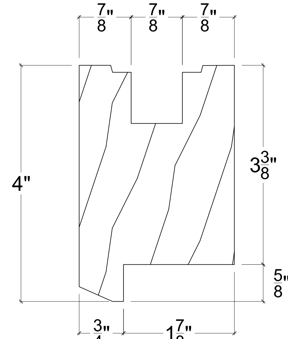
3A TOP RAIL - FIXED D8 1'-0" = 1'-0"
