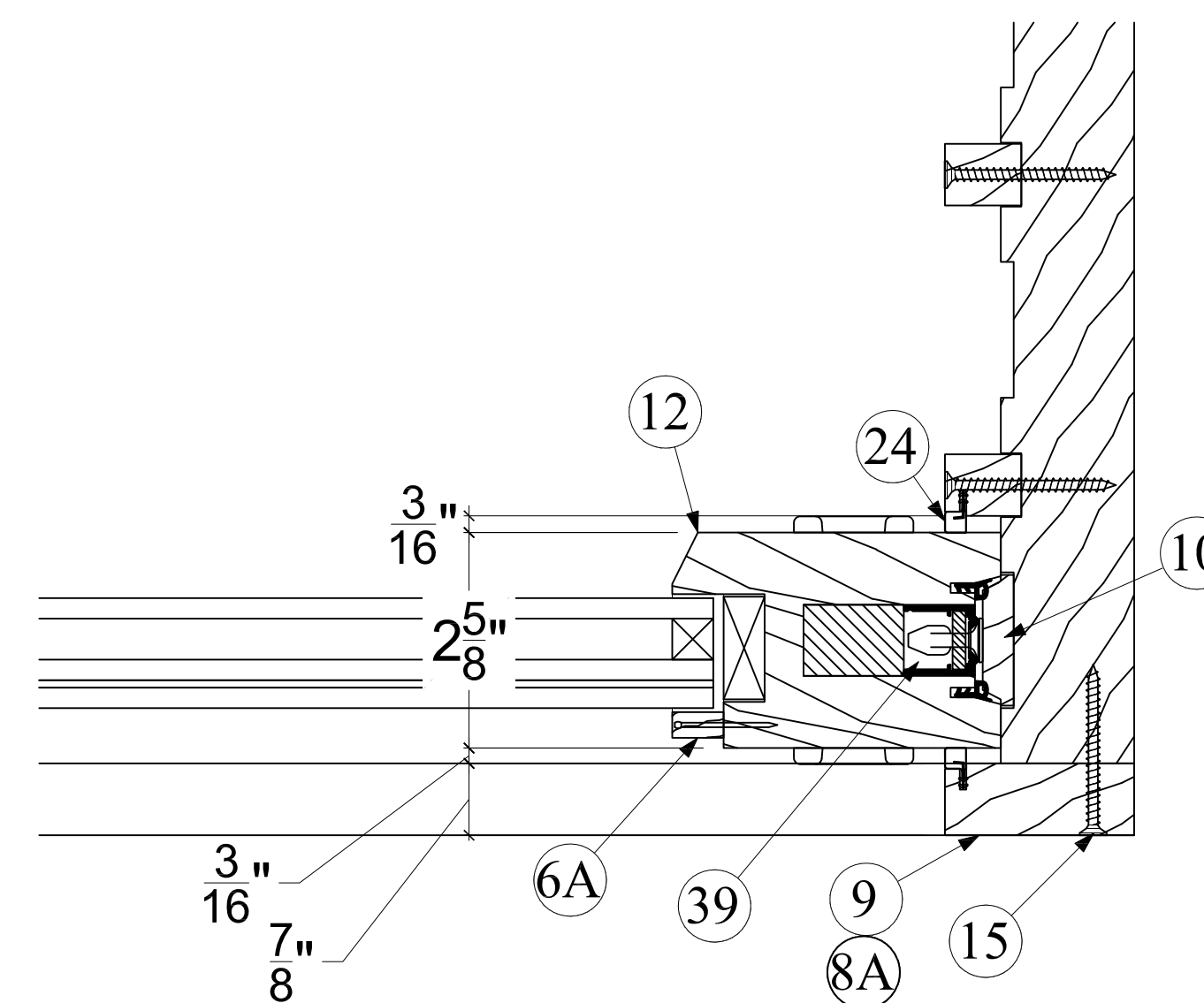
6 D5 LOCK JAMB (LOCK PANEL MAY BE AT ANY POSITION ON FRAME JAMB)
