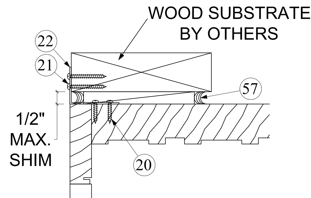
2 HEADER AND JAMB INSTALLATION, ANGLE CLIP D7 APPLIES TO INTERIOR AND/OR EXTERIOR OF FRAMING
