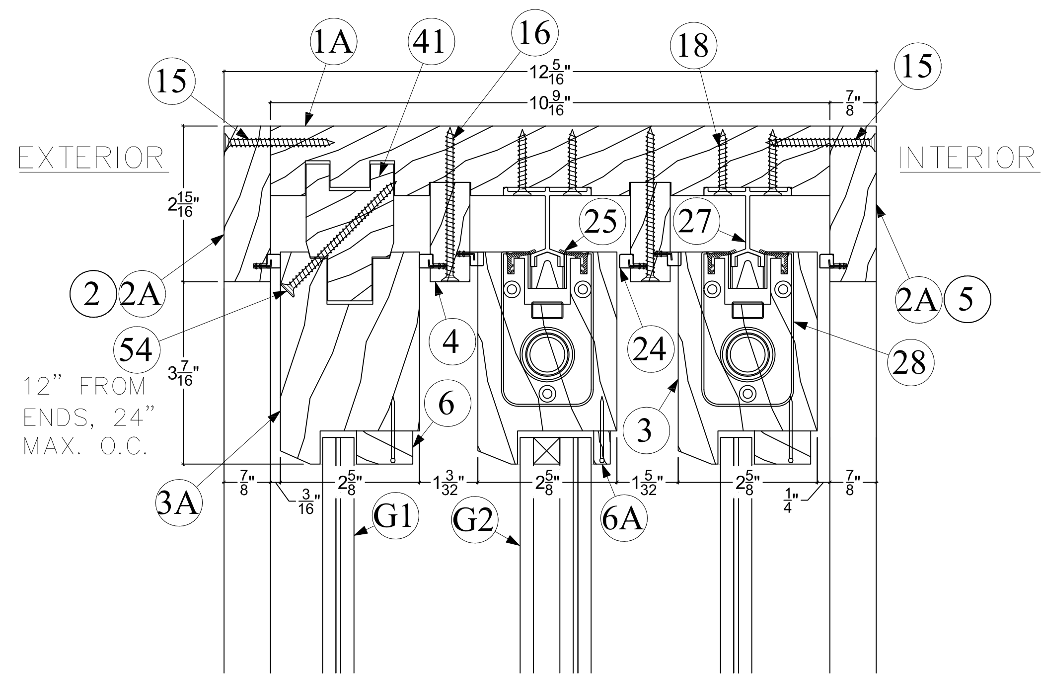
1 D5 LIFT AND SLIDE - HEAD DETAILS (3-TRACK OXX SHOWN) (HEAD DETAILS FOR OTHER CONFIGURATIONS SIMILAR)
