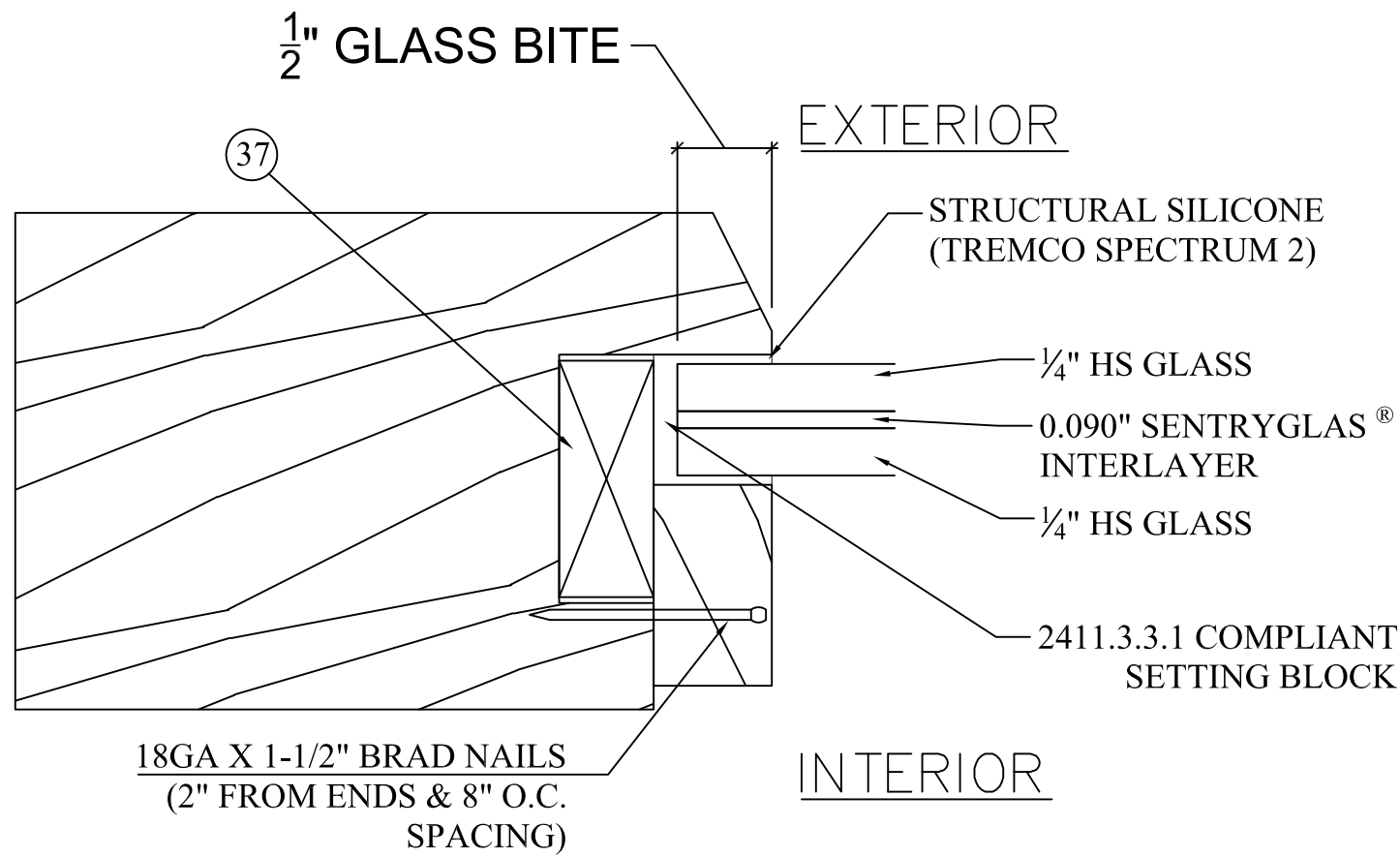
G1 GLAZING DETAILS - 9/16" LAMINATED GLASS D1 1'-0" = 1'-0"
