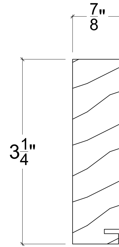
2 HEADER SASH STOP - EXTERIOR D8 1'-0" = 1'-0"
