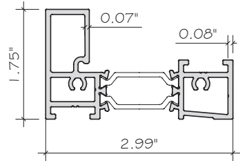
E35 SQUARED BEAD STD ES-P300-593 ALUM. 6063-T6
