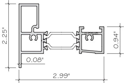
E32 SQUARED BEAD FLANGE ES-P300-607 ALUM. 6063-T6
