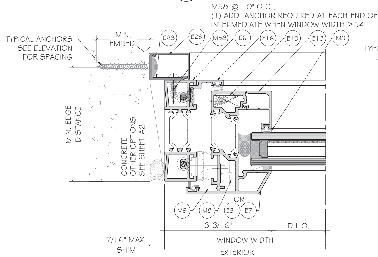
1 D6 DETAIL
