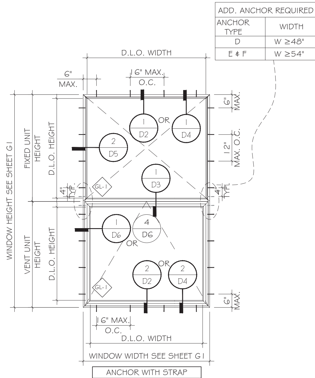
TYPICAL WINDOW ELEVATIONS
