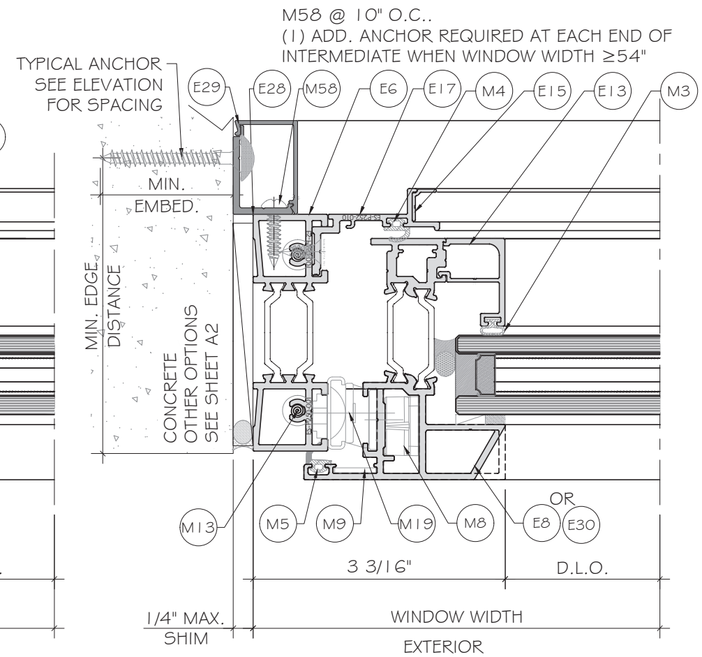
4 D6 DETAIL
