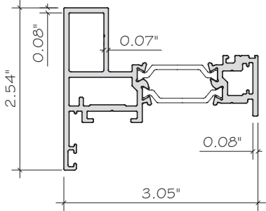
E30 SQUARE BEAD SASH ES-P300-603 ALUM. 6063-T6
