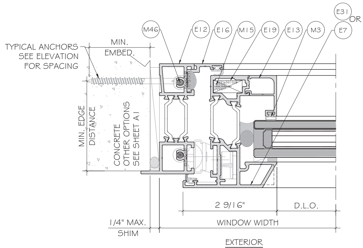
1 D7 DETAIL
