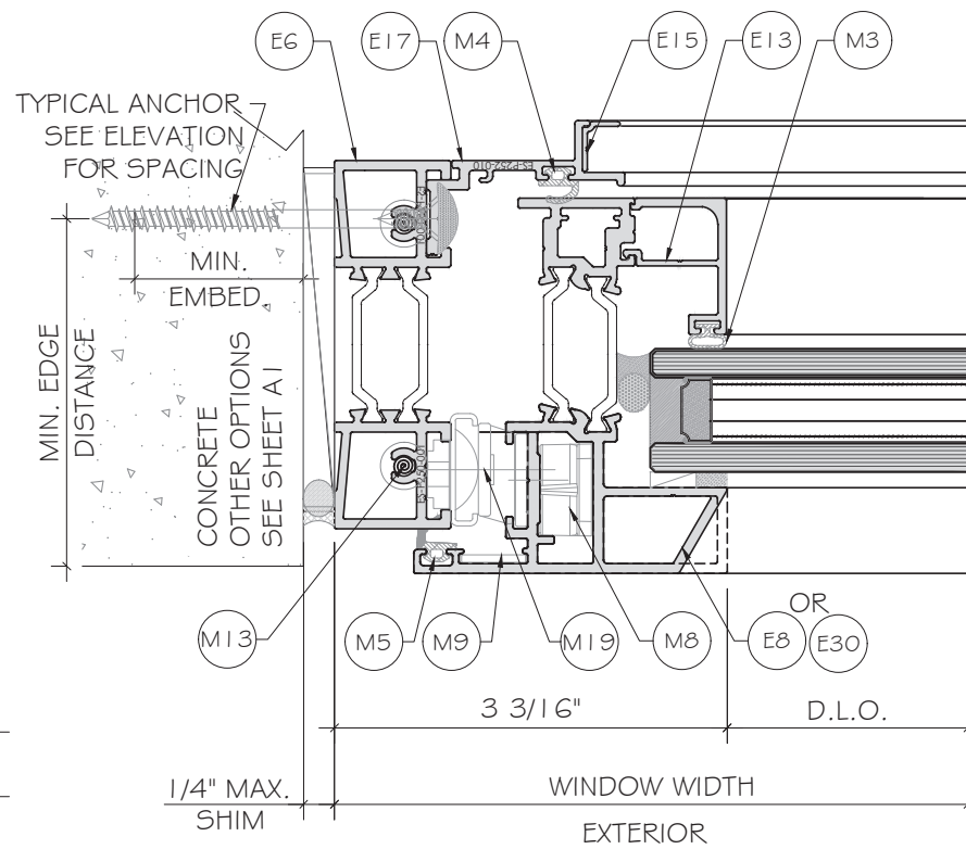
3 D6 DETAIL
