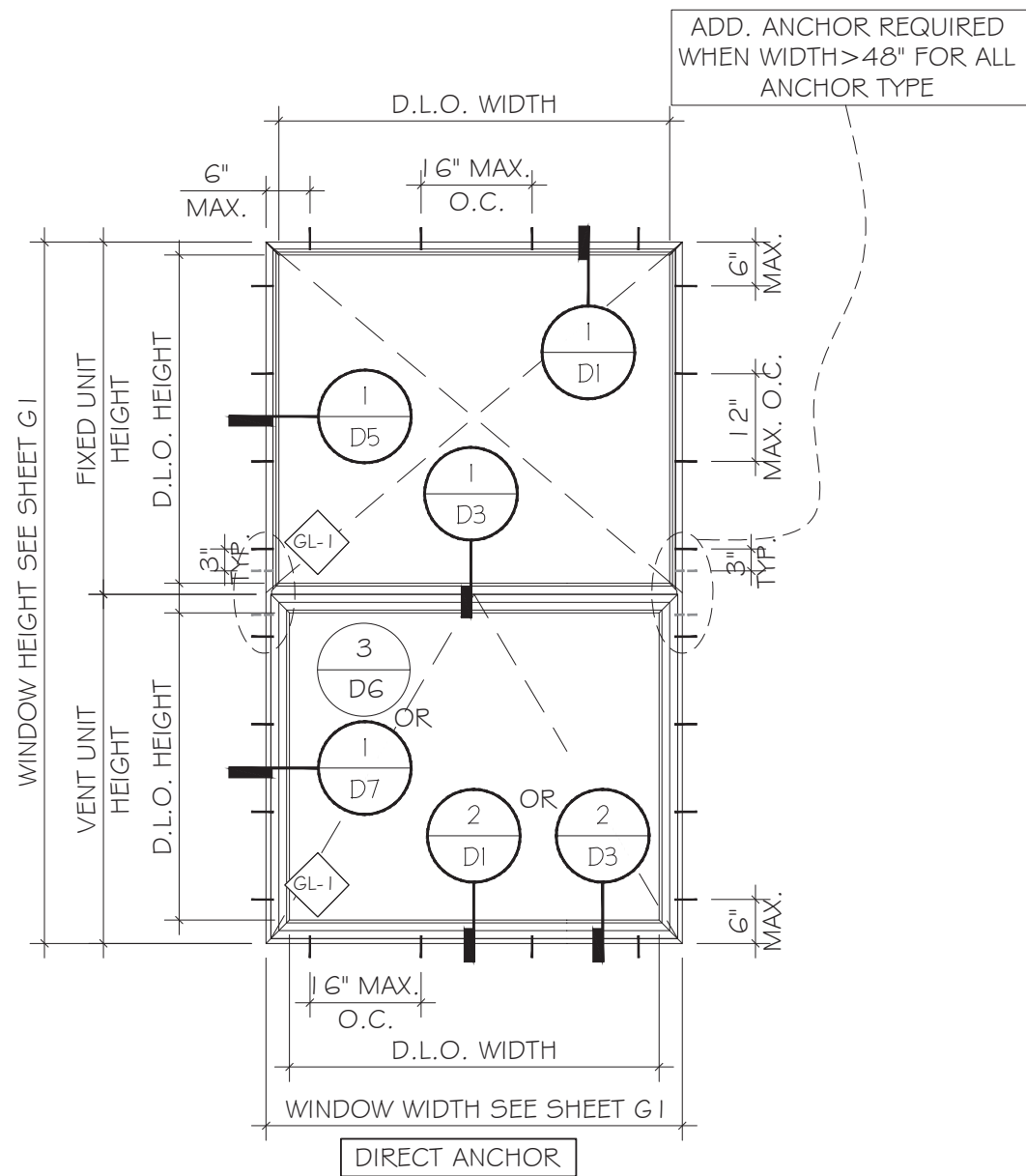
TYPICAL WINDOW ELEVATIONS
