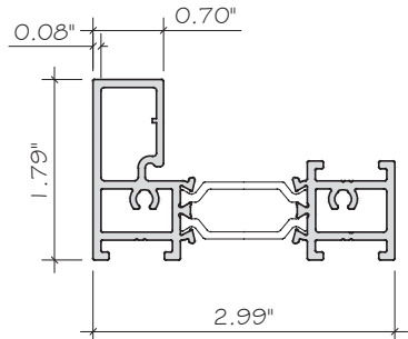
E36 INTERMEDIATE ES-P300-610 ALUM. 6063-T6
