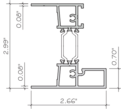
E33 SQUARED BEAD RECEPTOR ES-P300-606 ALUM. 6063-T6
