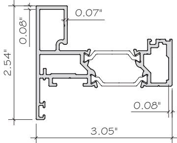
E31 SQUARE BEAD SASH ES-P300-602 ALUM. 6063-T6
