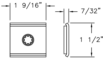
BACK PLATE STEEL
