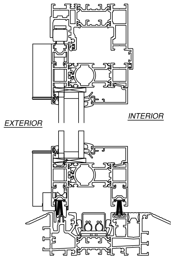
VERTICAL CROSS SECTION WITH SADDLE SILL
