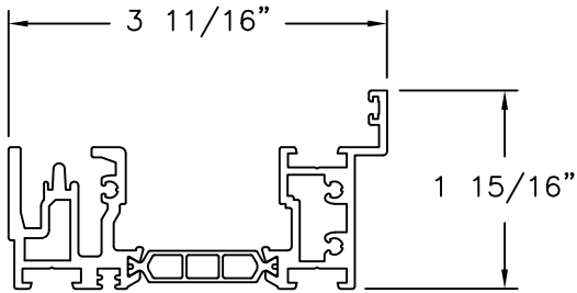
PERFORMANCE SILL PROFILE (5-320-08) ALUMINUM 6063-T5
