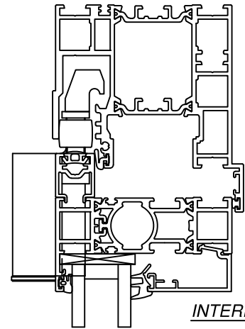
VERTICAL CROSS SECTION WITH EXTENDED HEAD AND FLUSH SILL
