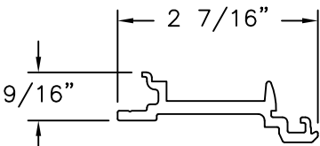
CONNECTION STRIP PROFILE (5-320-27) POLYAMIDE
