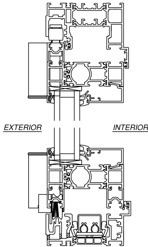
VERTICAL CROSS SECTION WITH PERFORMANCE SILL
