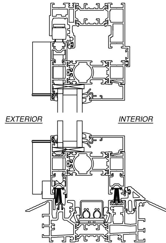
VERTICAL CROSS SECTION WITH UNIVERSILL
