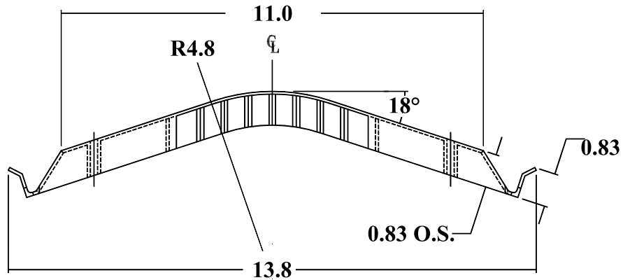
LOW PROFILE SHINGLE VENT II-11" and TRI-BUILT® 4' Ridge Vent with Filter
