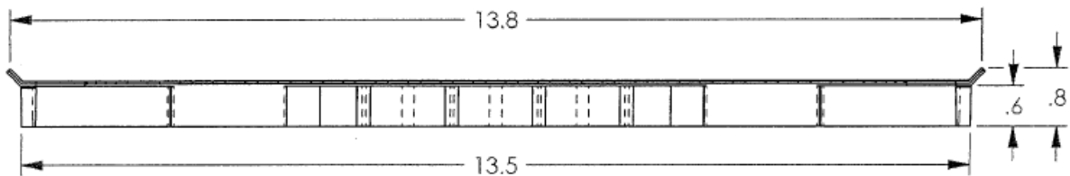
END VIEW
