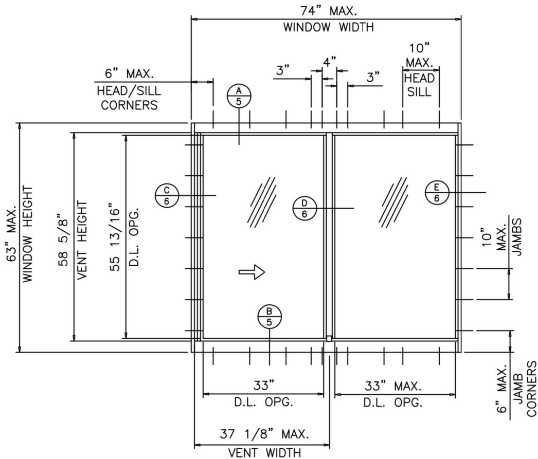
TYPICAL ELEVATION
