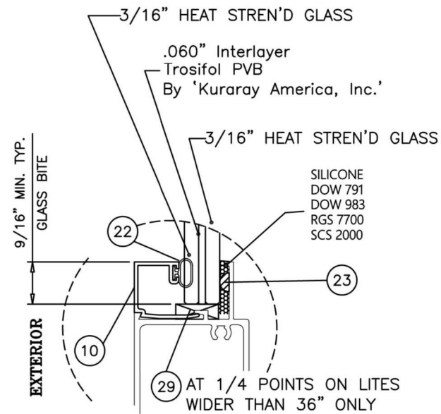
GLASS TYPE 'C' 7/16" OVERALL LAM. GLASS
