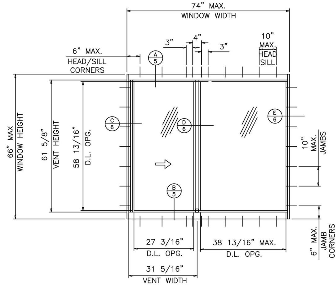
TYPICAL ELEVATION
